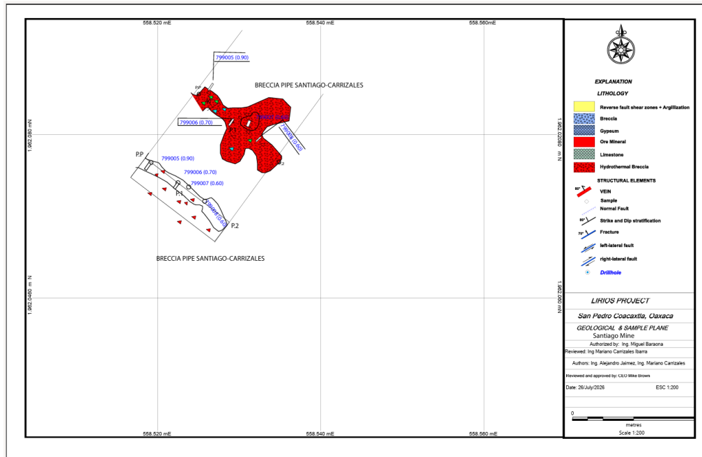
Figure 3: Geological map of the Santiago underground working illustrating the interpreted Santiago–Carrizales Breccia Pipe, channel sample locations and a longitudinal section
