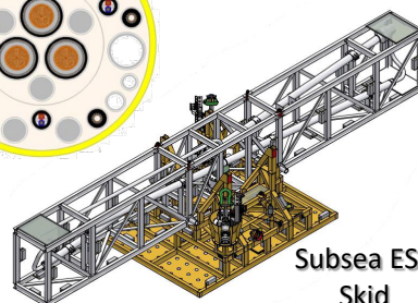
Umbilical Cross-section
