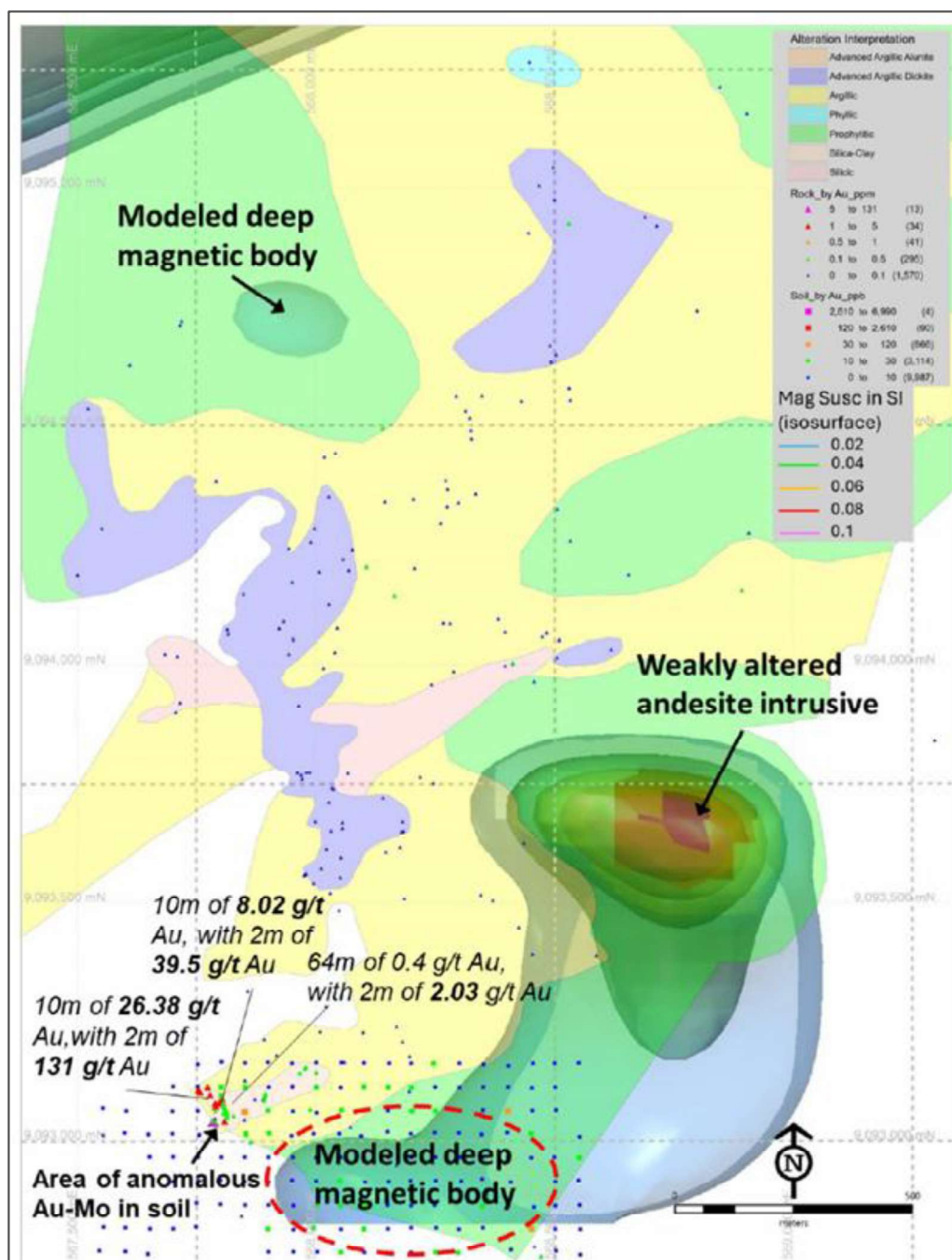
Figure 3.20: 3D magnetic inversion modelling at the Ngerdani prospect
