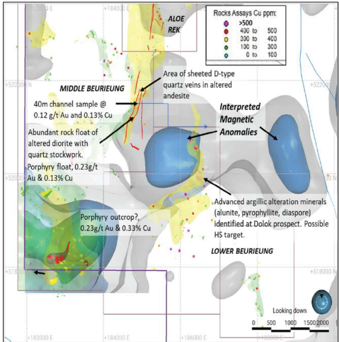
Figure 3.12: Beurieung prospect
