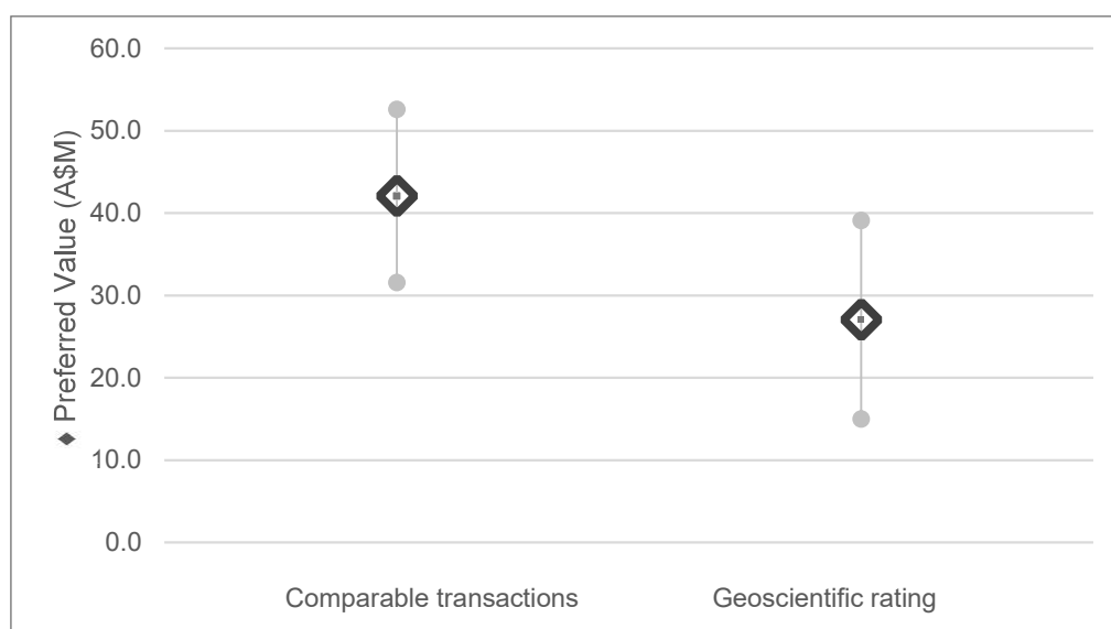
Figure 6.5: Exploration potential value range of valuation methods
