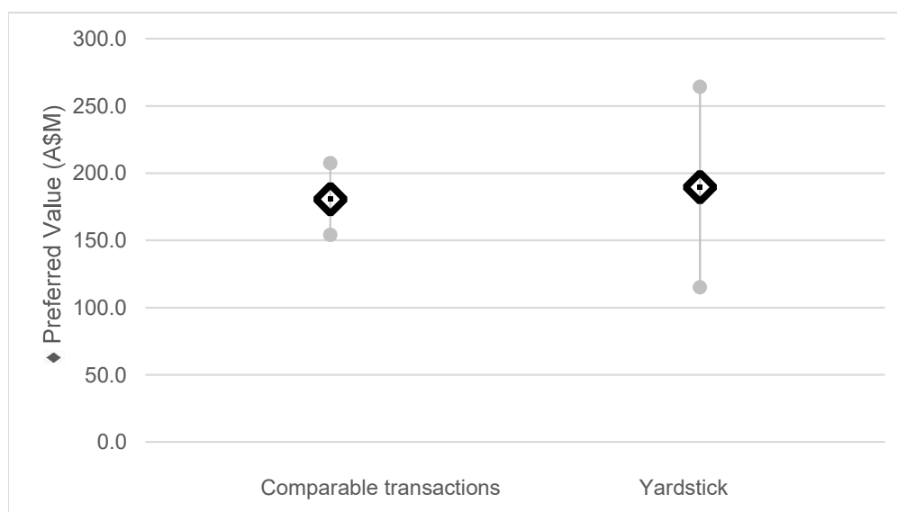
Figure 6.2: Summary of valuation methods of total 100% value – Mineral Resources
