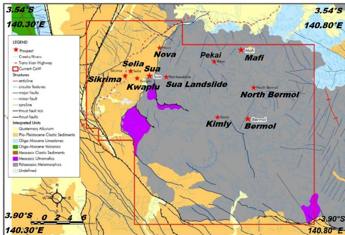
Figure 3.3: Idenburg project geology
