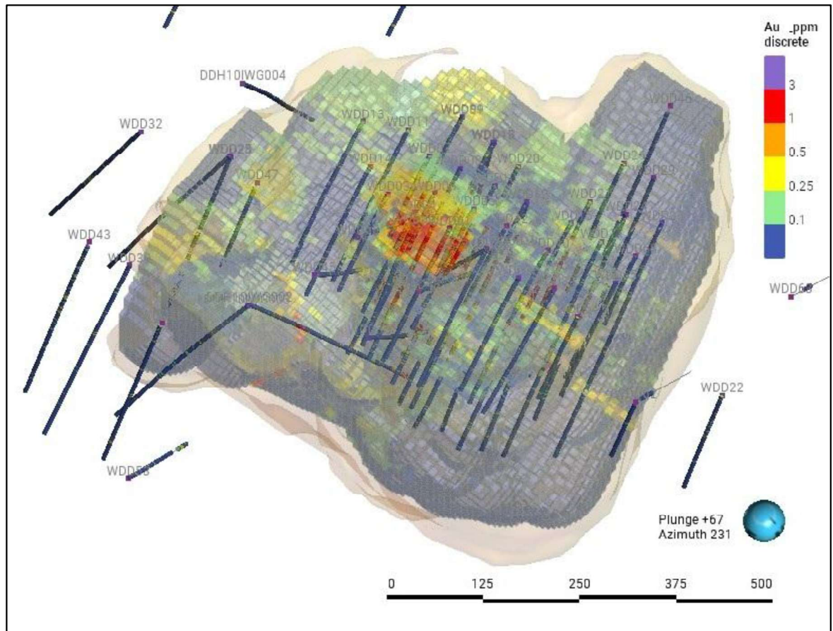
Figure 3.23: Mineralised domains of Wonogiri project
