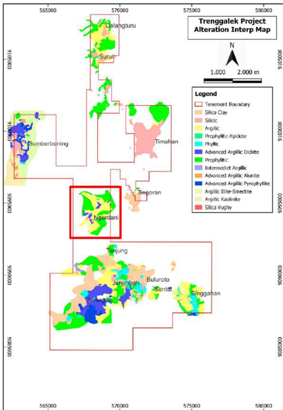
Figure 3.15: Trenggalek prospects
