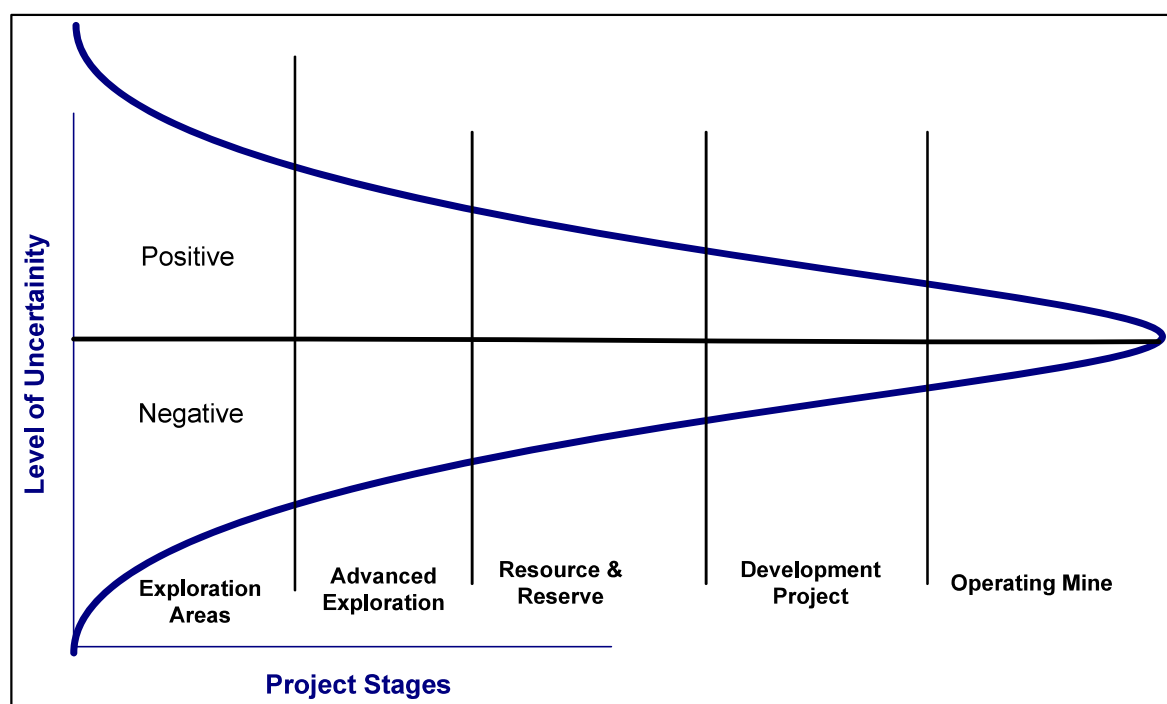
Figure 6.6: Uncertainty by advancing exploration stage
