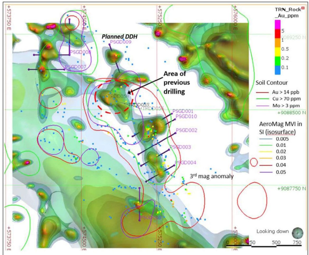
Figure 3.16: Singgahan prospect
