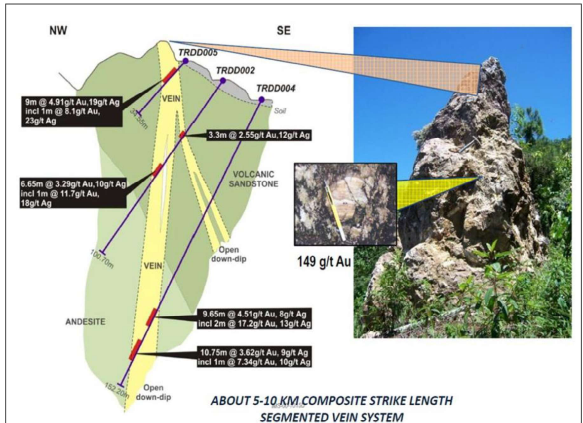
Figure 3.18: Sentul prospect
