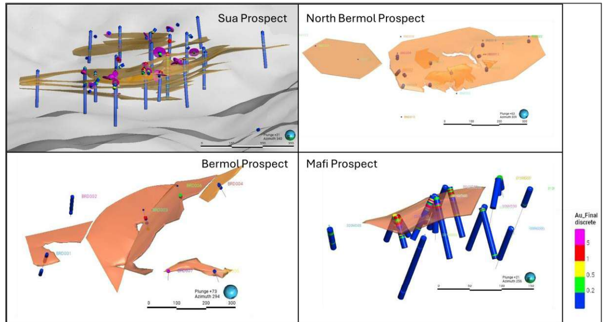
Figure 3.4: Mineralised domains of Sua, Bermol, North Bermol and Mafi prospects
