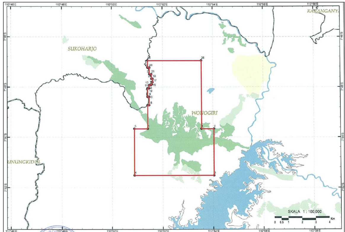
Figure 3.22: Concession map of Wonogiri project
