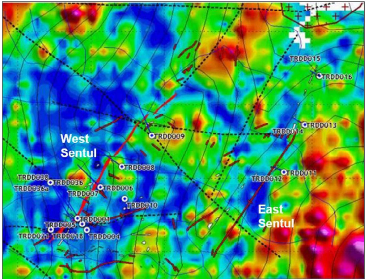
Figure 3.19: Historical drill hole locations targeting the Sentul prospect
