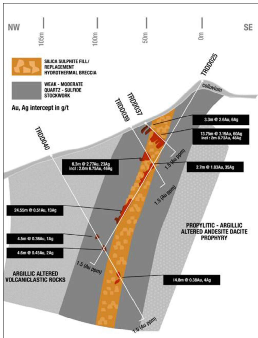
Figure 3.17: Reconnaissance drilling across breccia zone at the Buluroto prospect
