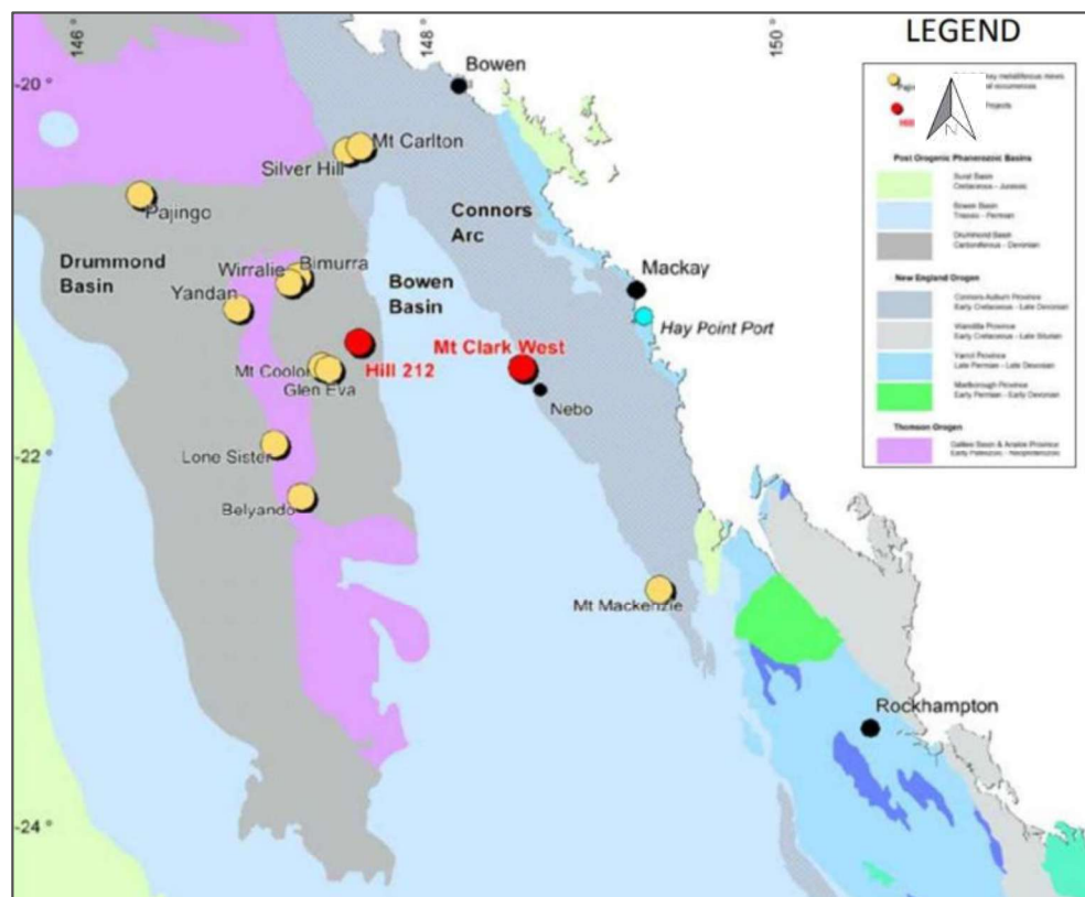
Figure 4.3: Regional geological map of Mount Clark West project
