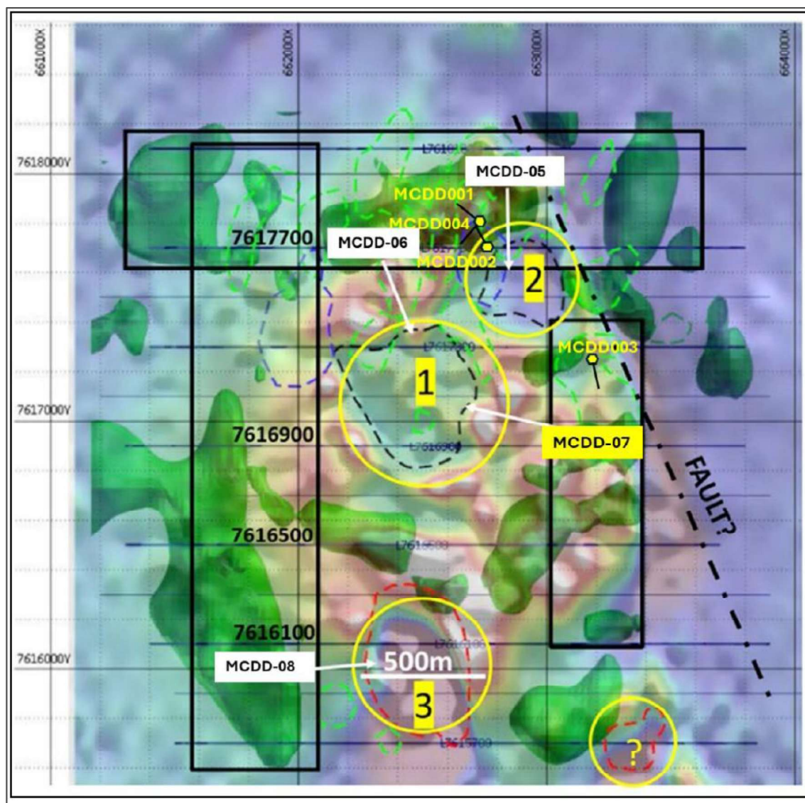
Figure 4.4: Interpreted RTP magnetic image base with interpreted MIMDAS zones of high chargeability (green)
