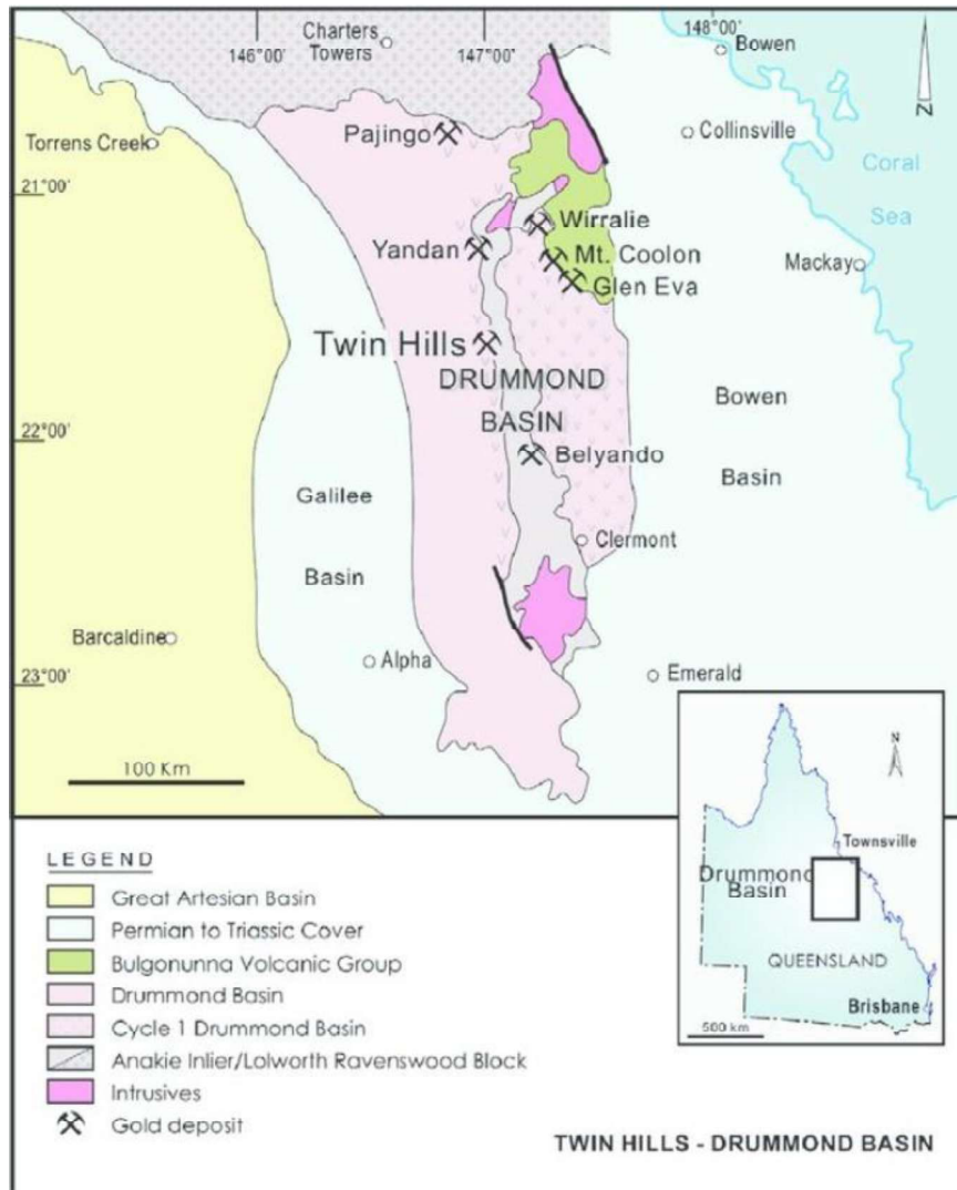
Figure 4.2: Drummond Basin regional geology
