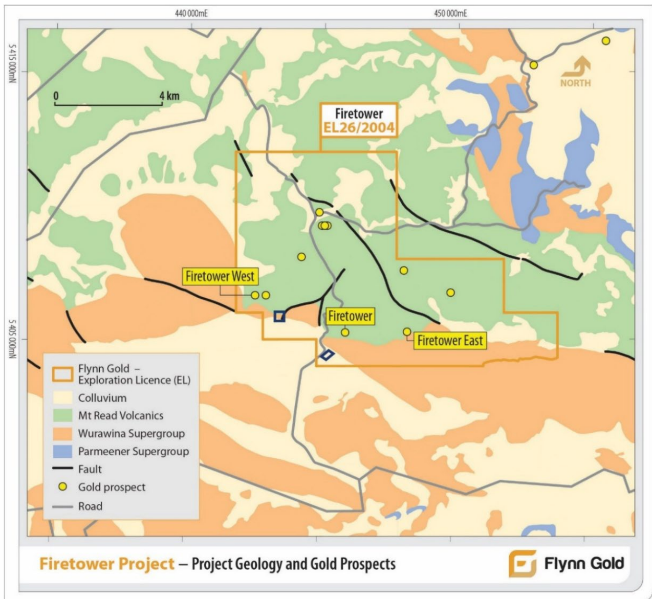
Figure 6 – Firetower Project Simplified Geology And Gold Prospects
