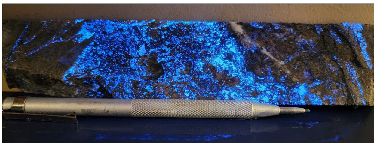
Figure 4 – Same segment of drill core (2019FTD007E, 129.8m) under ultraviolet light, highlighting intense scheelite (CaWO 4 ) mineralisation (blue) (Interval 129.5-130.0m Assay: 0.5m @ 6.64g/t Au, 0.38% Co, 3.79% WO 3 , 0.11% Cu).
