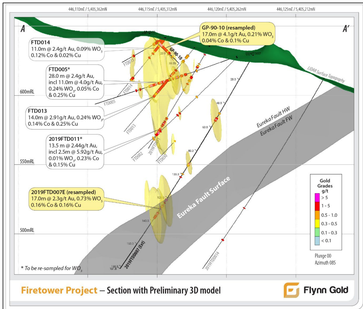
Figure 1 –Cross Section with preliminary 3D model of the Firetower Prospect (looking east).
