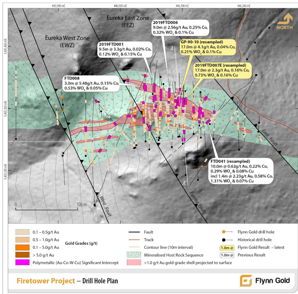
Figure 2 - Firetower Prospect Drill Hole Location Plan.
