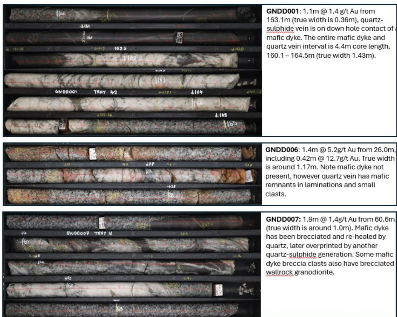
Figure 4 – Core photos showing quartz veins and associated mafic dykes.
