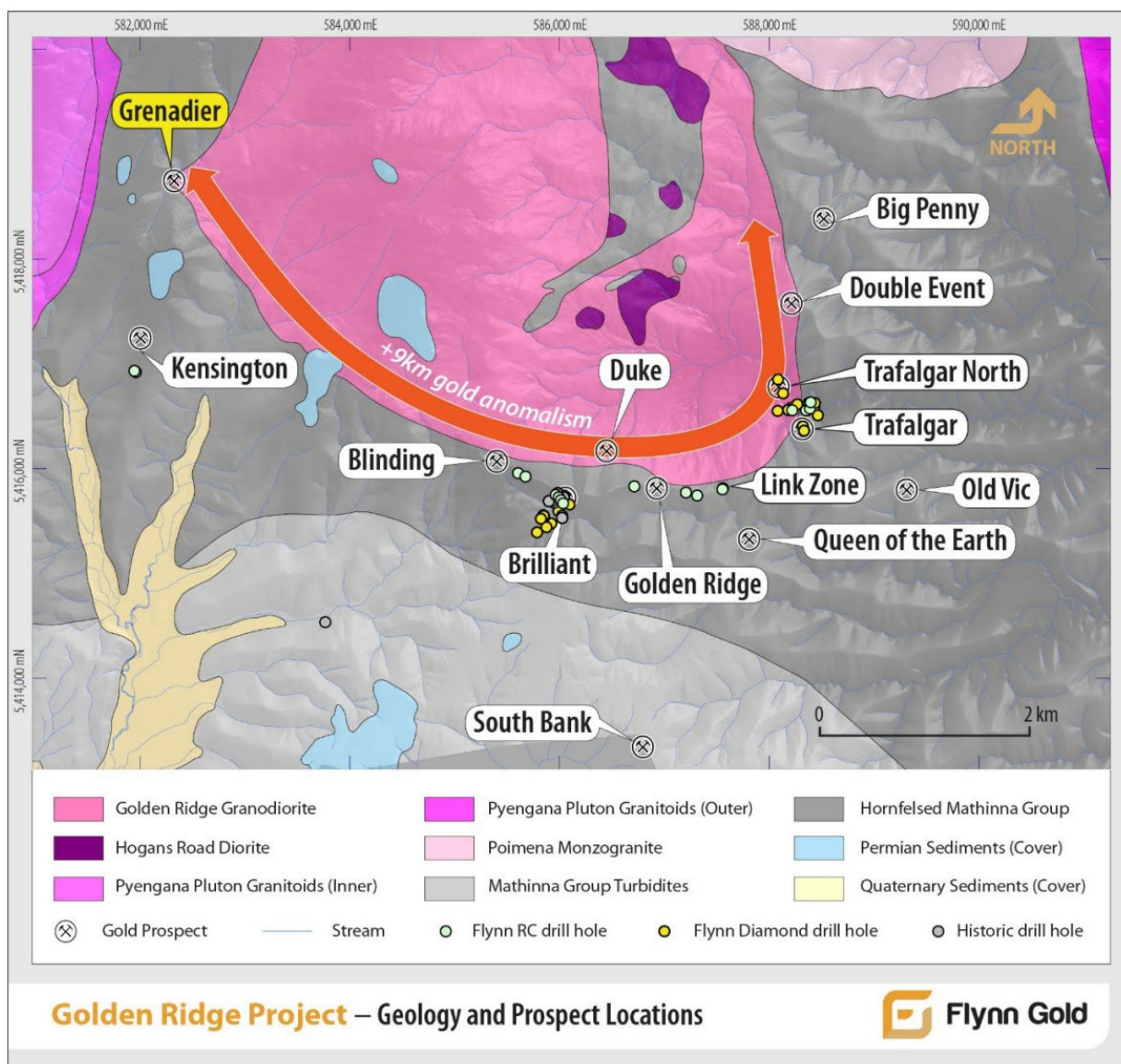
Figure 7 – Golden Ridge Project – Geology and Prospect Locations.
