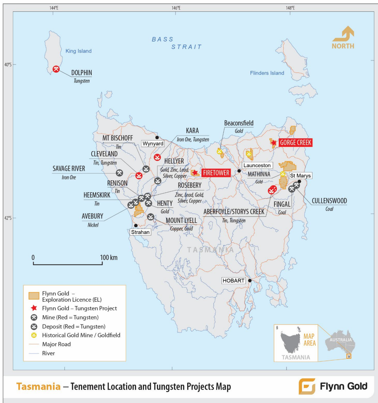
Figure 4 – Location of Flynn Gold tenements in Tasmania.
