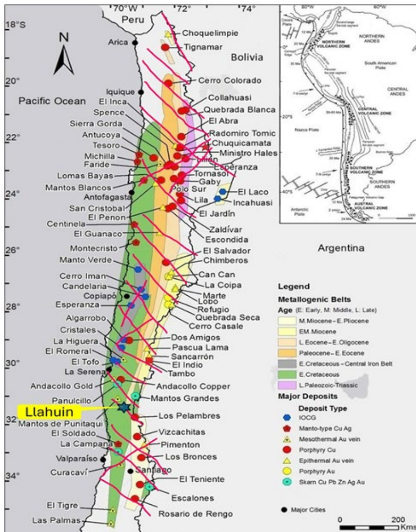
Figure 5. Central and Northern Chile with the Llahuin Project showing metallogenic belts, significant deposits, and interpreted structures.
