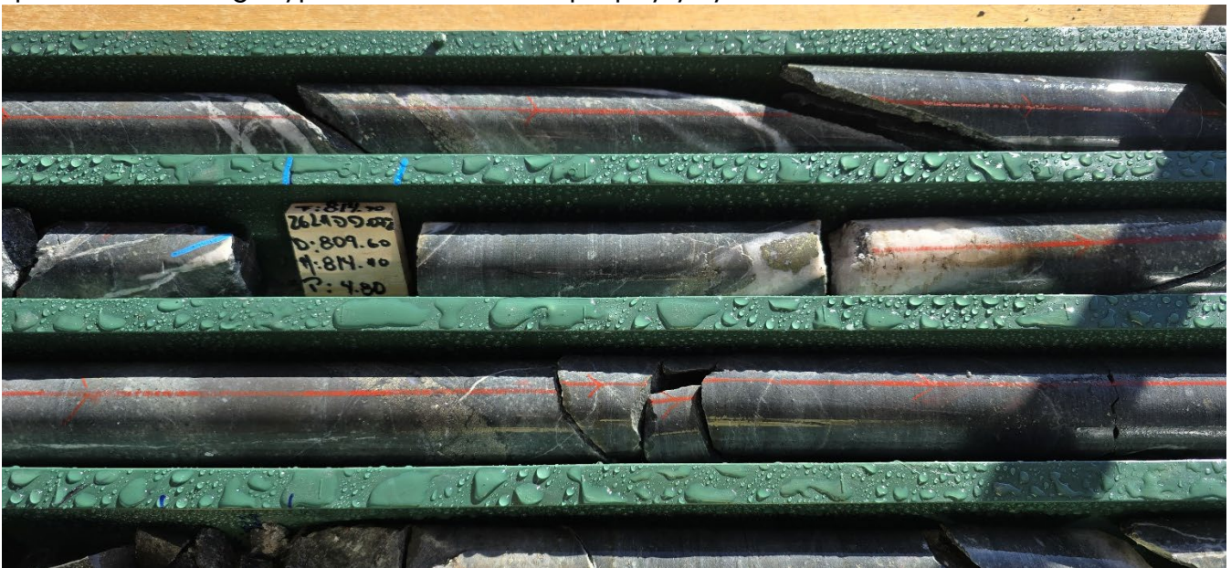
Photo 2. Zone of intense pyrite-chalcopyrite-quartz vein style and fine disseminated mineralisation from 809m downhole in 26LHDD072* (refer to Appendix 1).
