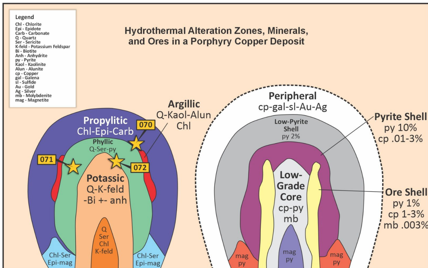
Figure 3. Hydrothermal alteration zones associated with porphyry copper deposit (modified after Lowell & Guilbert 1970) with interpreted locations of completed FMR drillholes 25LHDD070, 25LHDD071, and 26LHDD072.
