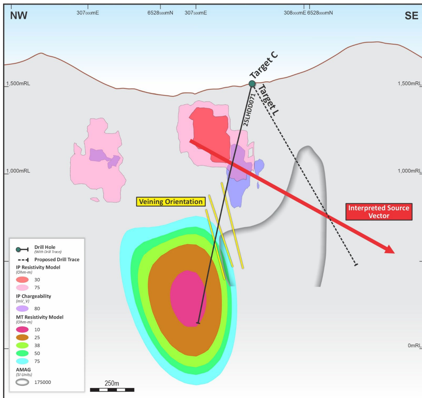
Figure 2. Cross section L-L', Target L, showing geophysical models and proposed drillhole to 1,200m downhole depth, testing new structural and geochemical vectors east of Target C and south of Target K (+/- 10m window).*
