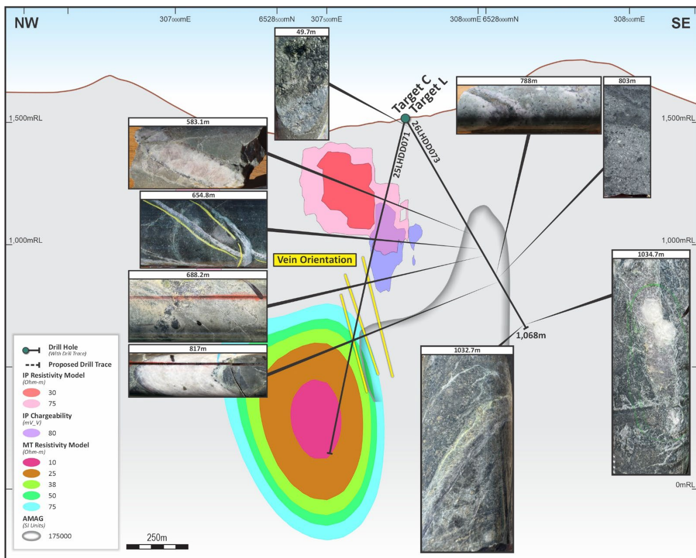
Figure 2. Cross section L-L', Target L – 26LHDD073, showing geophysical models and completed drillhole to 1,068.0m downhole depth, including mid-level shallow IP Resistivity and IP Chargeability features and the large MT high amplitude feature at depth (+/- 10m window)* intersected in 25LHDD071 and interpreted as pyrite rich peripheral mineralisation. The mineralisation photographs are of sooty chalcocite at 49.7m, molybdenite in anhydrite vein 583.1m, molybdenite in quartz vein 654.8m, chalcopyrite in matrix 688.2m, chalcopyrite in quartz 788m, chalcopyrite in magnetite vein 803m, molybdenite in quartz vein 817m, chalcopyrite in sulphide vein 1032.7m and in quartz-anhydrite vein at 1034.7m.
