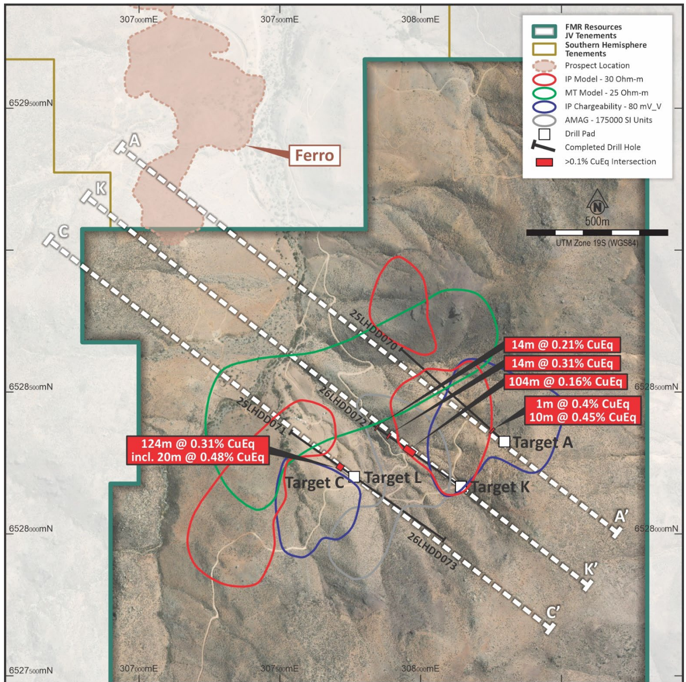
Figure 2. Plan view of Southern Porphyry, showing surface projections of geophysical models, completed drill targets and assay results to date*.
