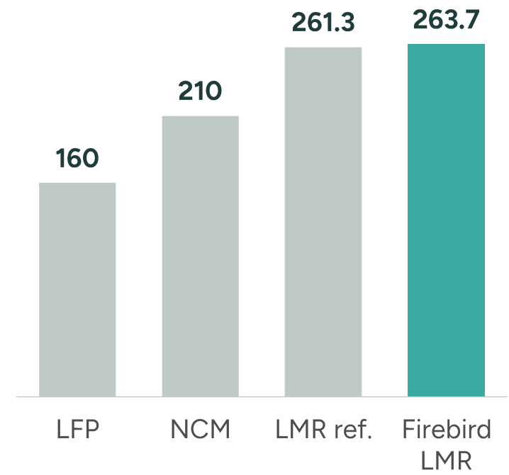
0.1C discharge capacity (mAh/g)
