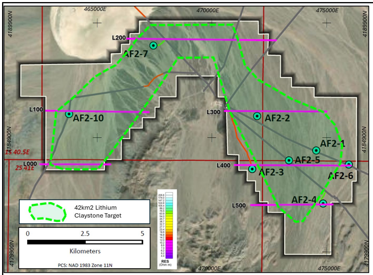
Figure 4. GEOPHYSICALLY DEFINED LITHIUM CLAYSTONE TARGET
