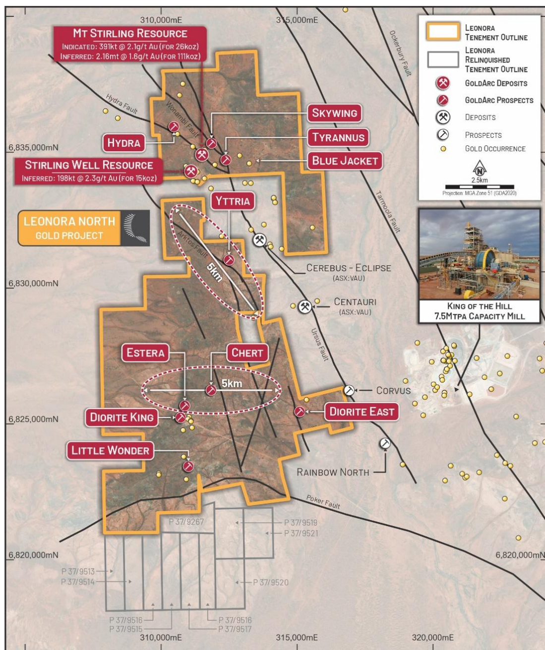
Figure 5 – Leonora North Gold Project Overview – Showing Yttria Prospect
