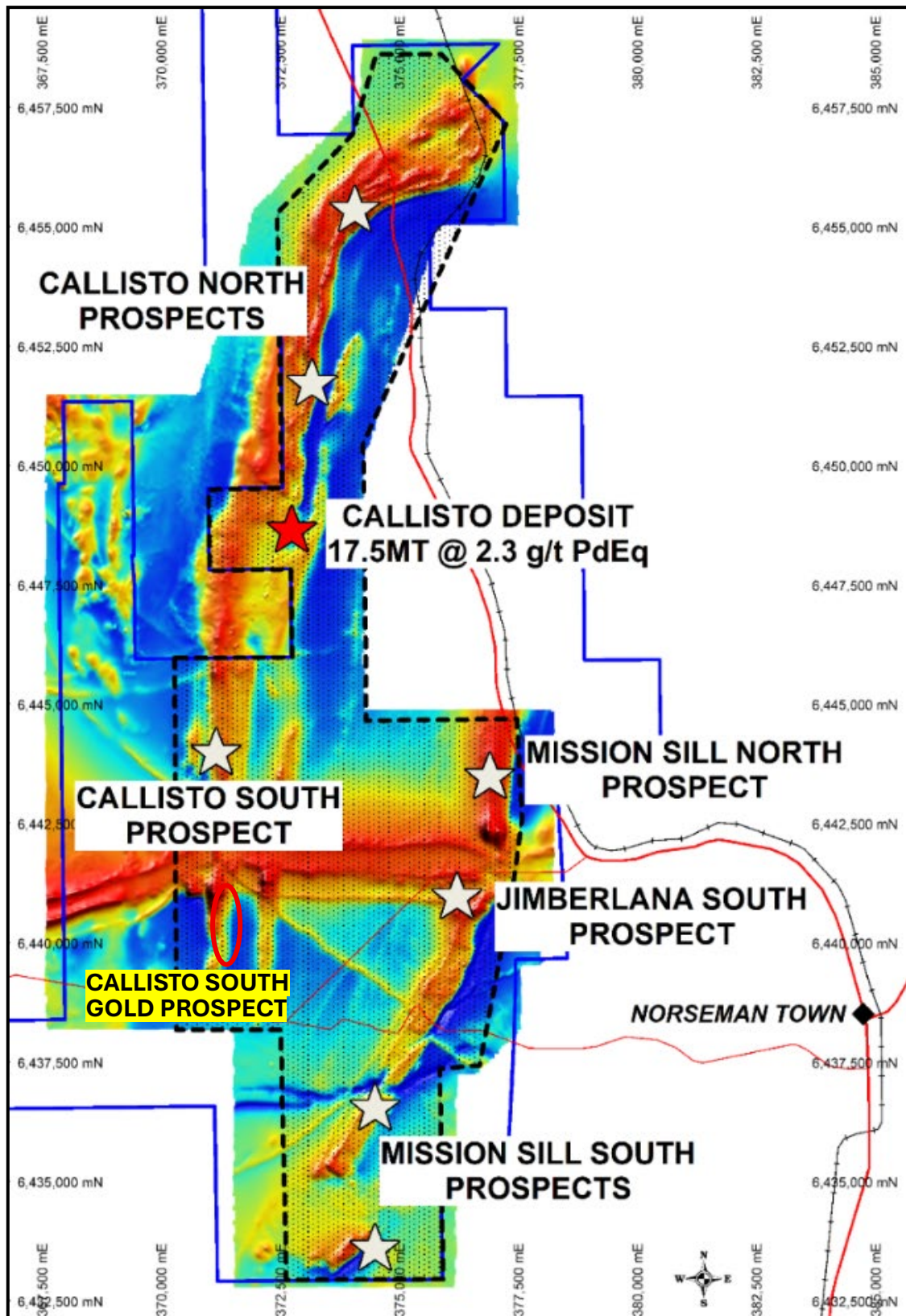
Figure 3 – Norseman Project outline (blue line) with gravity survey (black dashed line), Callisto Deposit (red star), and prospects requiring follow up drilling (grey stars). New gold prospect at Callisto South is shown by red ellipse.
