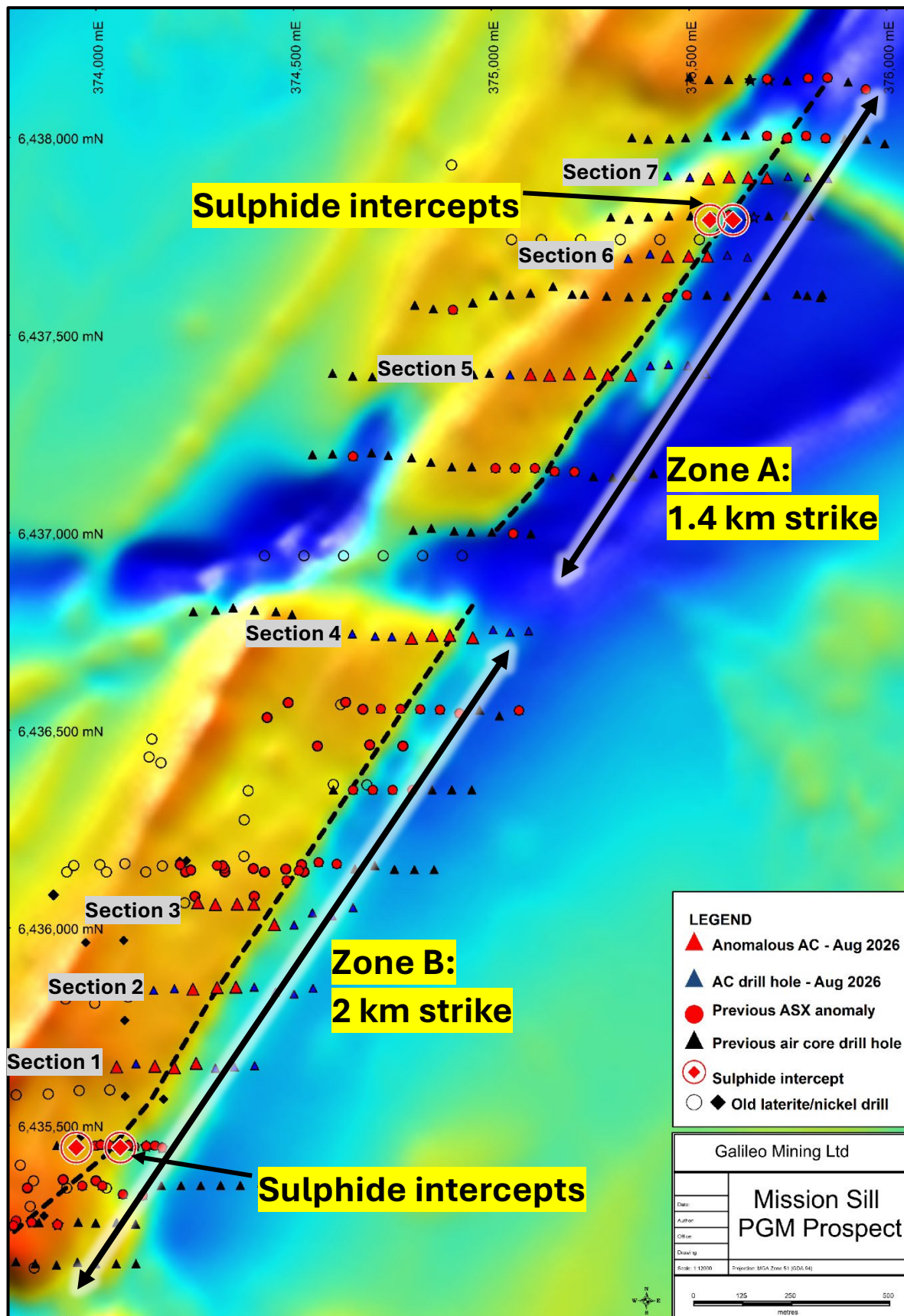
Figure 1 – Mission Sill AC drilling with anomalous drill holes, mineralisation trend (dashed lines), and sulphide intercepts (announced 19/03/26). Listed sections of recent drilling are included in the appendices. TMI magnetic background. See Appendices for drilling details.
