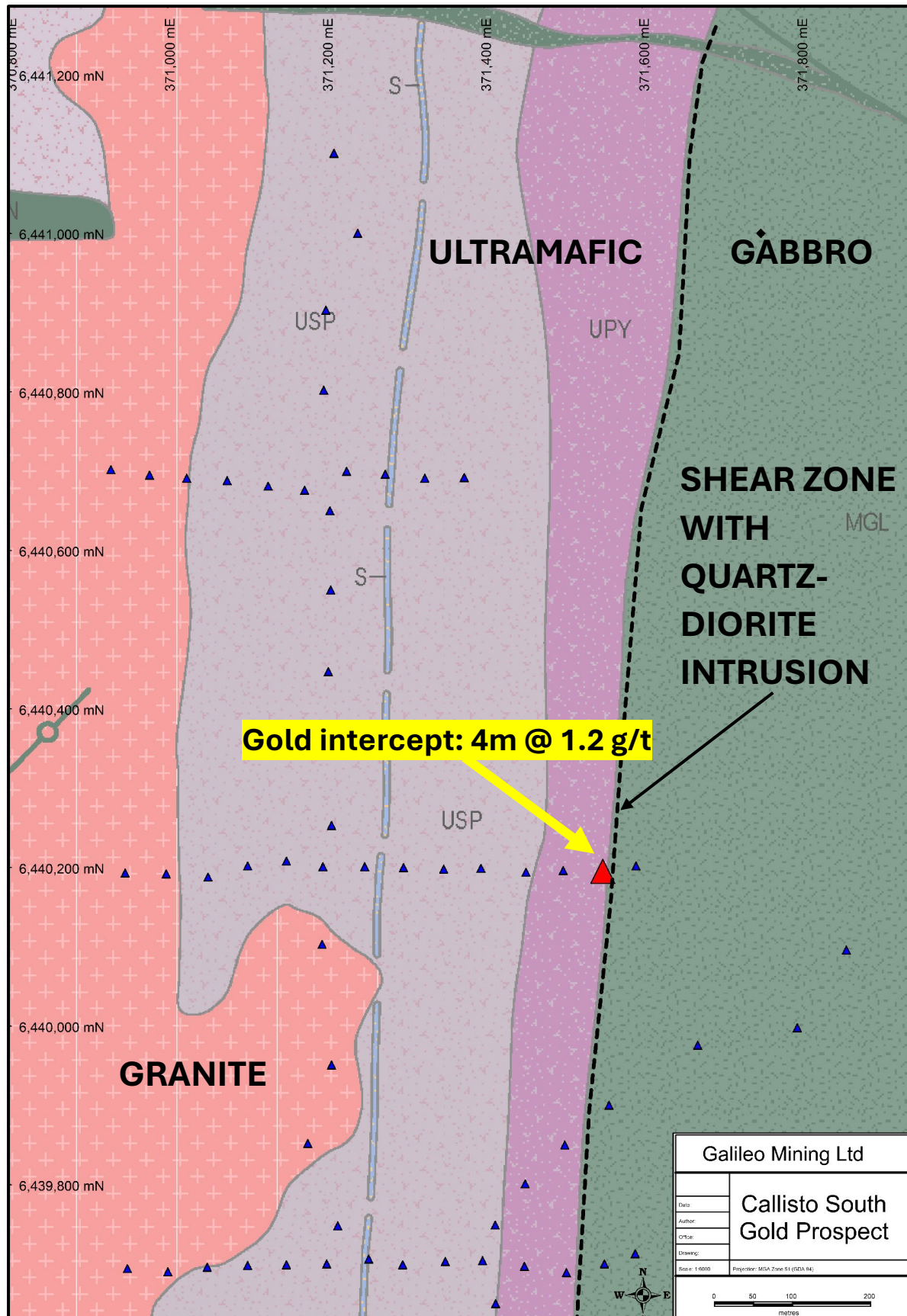
Figure 2 – Callisto South gold prospect with air core drilling (triangles), gold drill intersection, 10k mapped geology and interpreted shear zone. See Appendices for drilling details.
