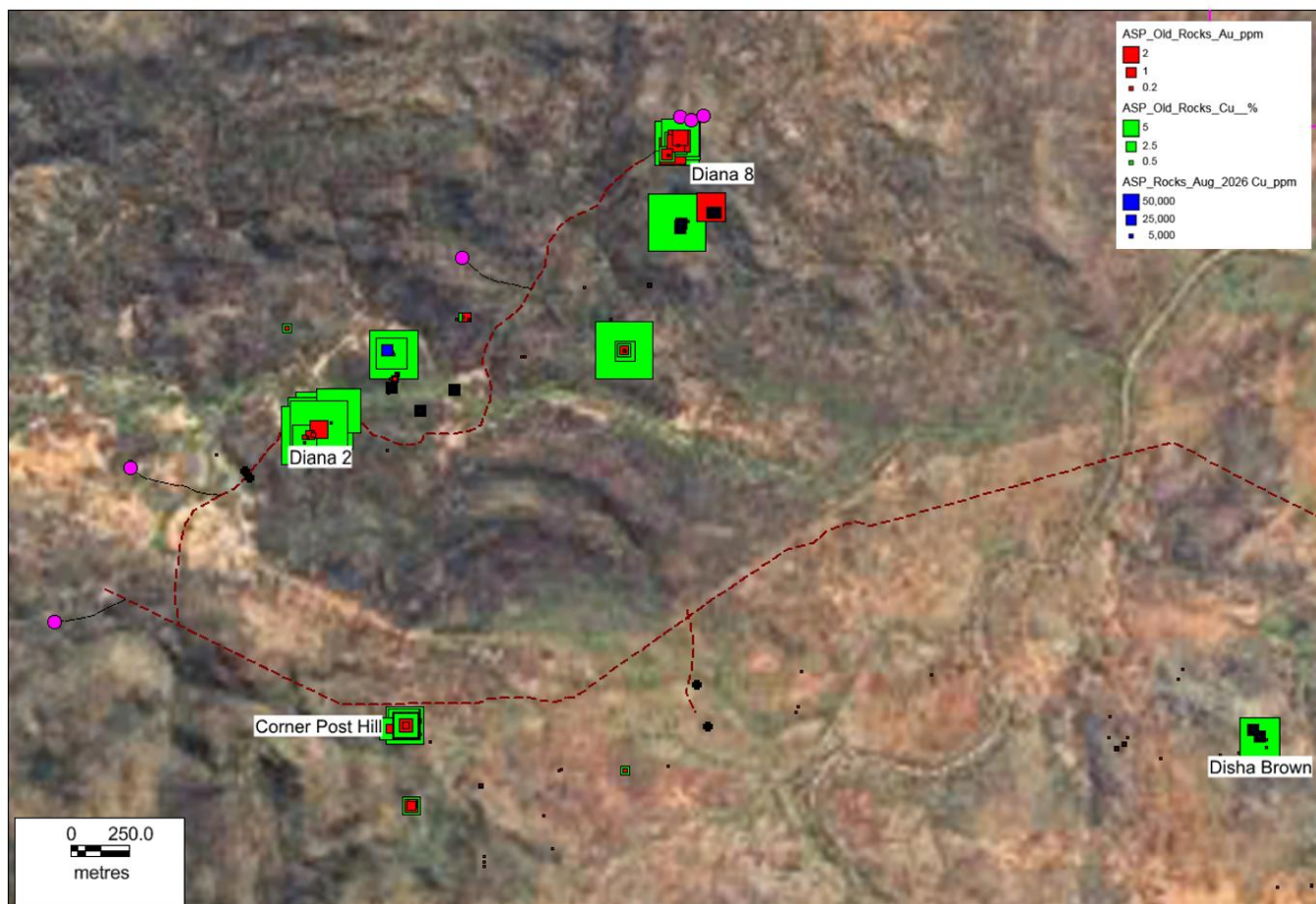
Figure 7 (above) Rock chip results at Alice Springs EL (Black squares). Only one significant sample (Blue square NE of Diana 2 Prospect). Old Genesis collars shown in Pink.
