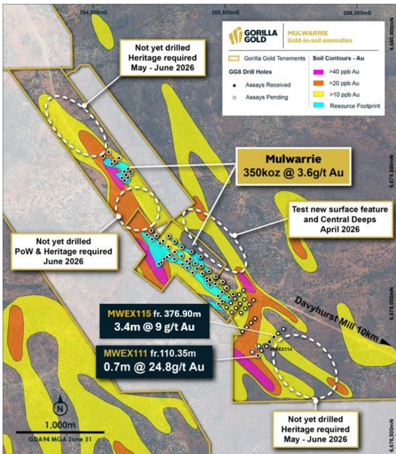
Figure 3. Gold-in-soil anomalies adjacent to the August 2025 MRE at Mulwarrie.
