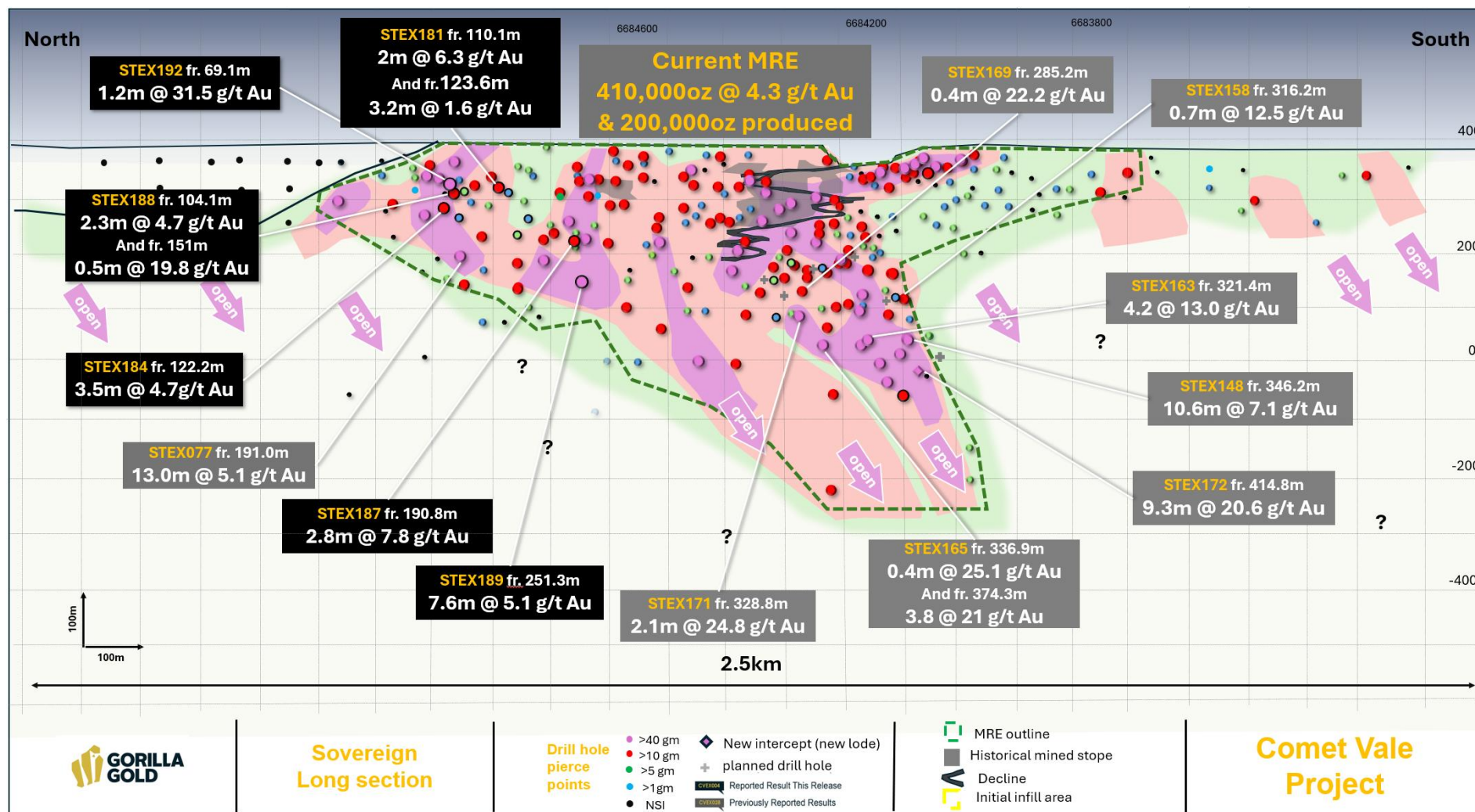
Figure 1. Sovereign Deposit Long Section.
