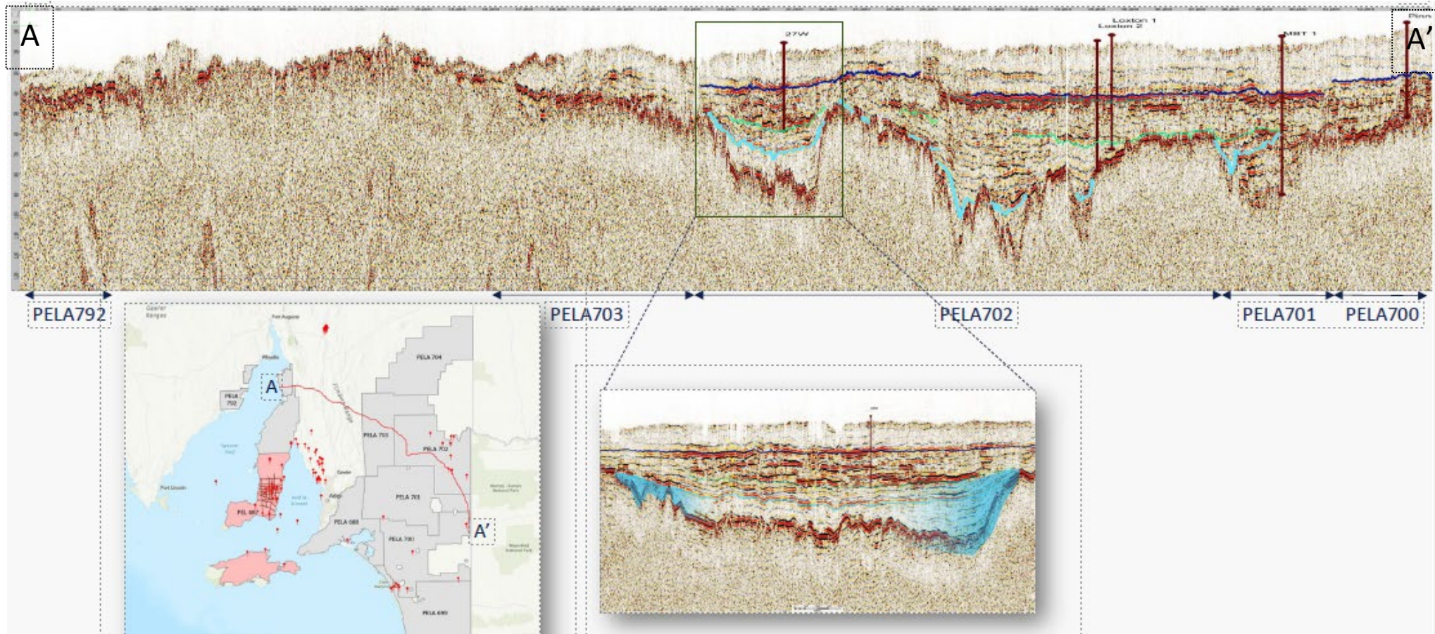
Figure 4: Cross Section of the Geoscience Australia Seismic Line Traversing Part of the Group's Application Areas
