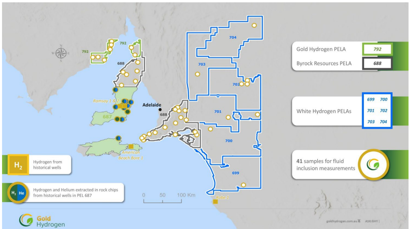
Figure 2: Map showing the fluid inclusion study points across the group's application areas.
