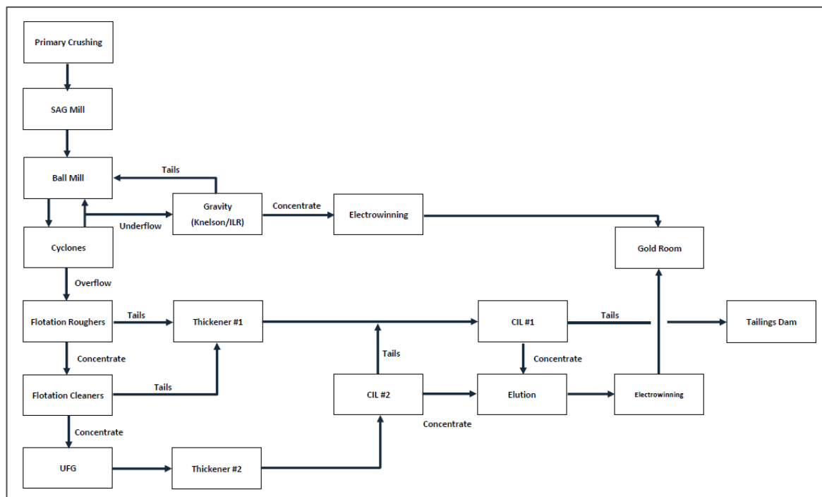
Figure 3.16: Lady Julie process flowsheet
