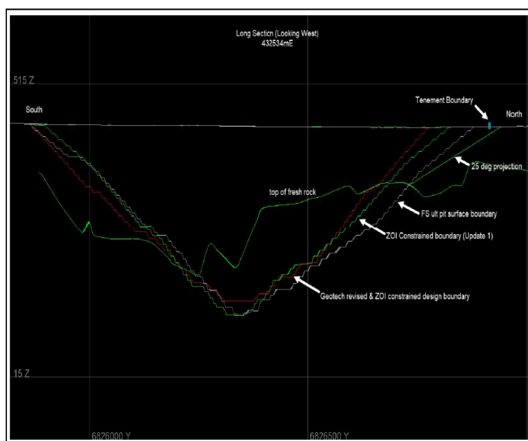
Figure 3.11: Lady Julie North open pit adjusted geotechnical impact
