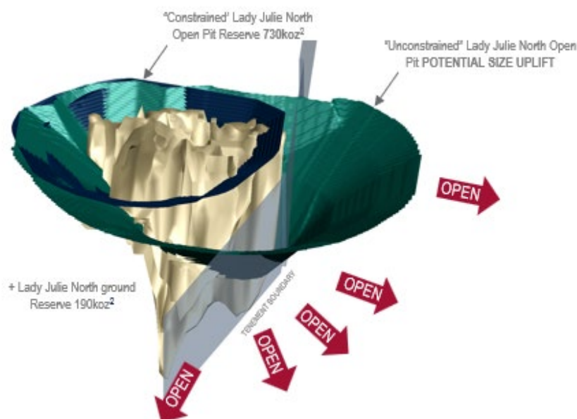
Figure 8 – Isometric view of Lady Julie pit optimisation ($3,500/oz gold price assumption)
