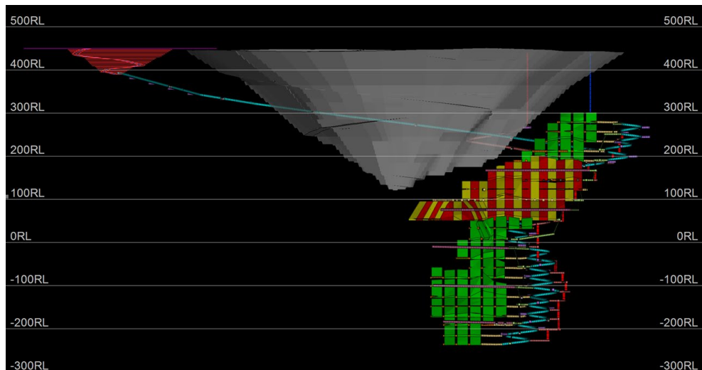
Figure 4 - LNJ4 Underground Section View Looking West
