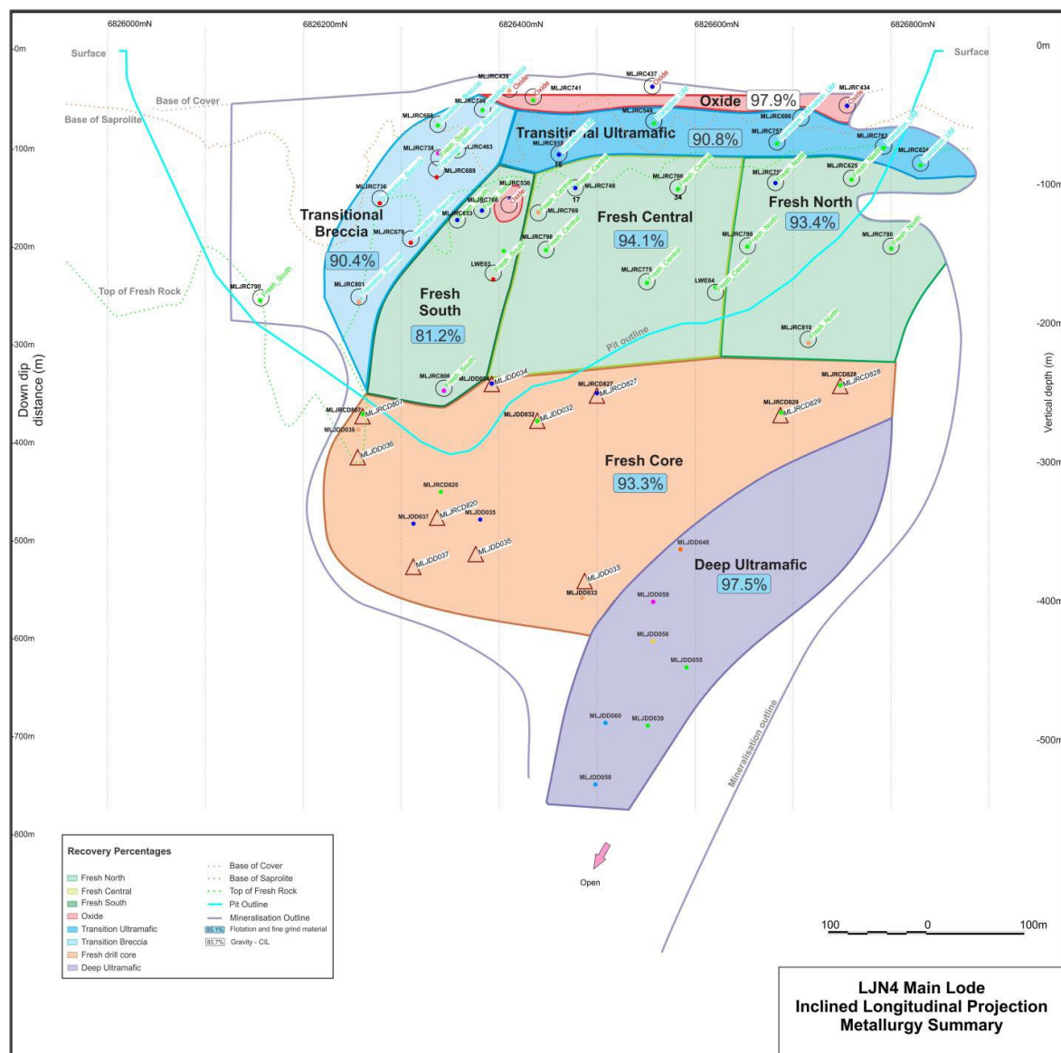
Figure 3.15: LJV4 eight metallurgical samples mineralisation types
