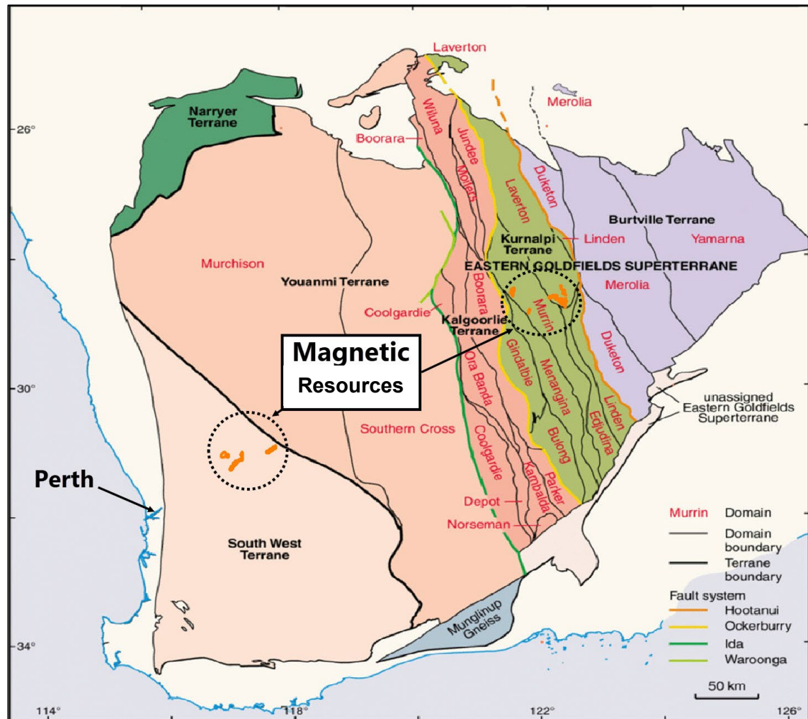
Figure 3.2: Regional setting
