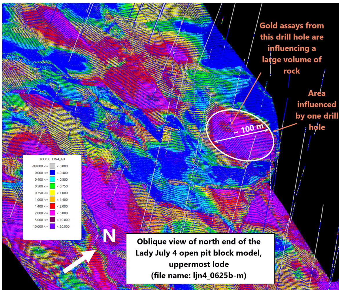
Figure 3.4: Lady Julie North 4 gold grades in Inferred
