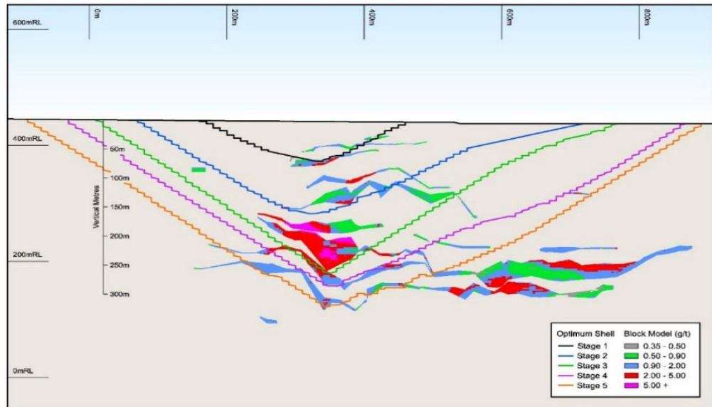
Figure 3 - LNJ4 starter pit and cutbacks
