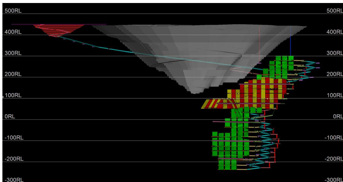
Figure 3.12: Lady Julie underground mine design
