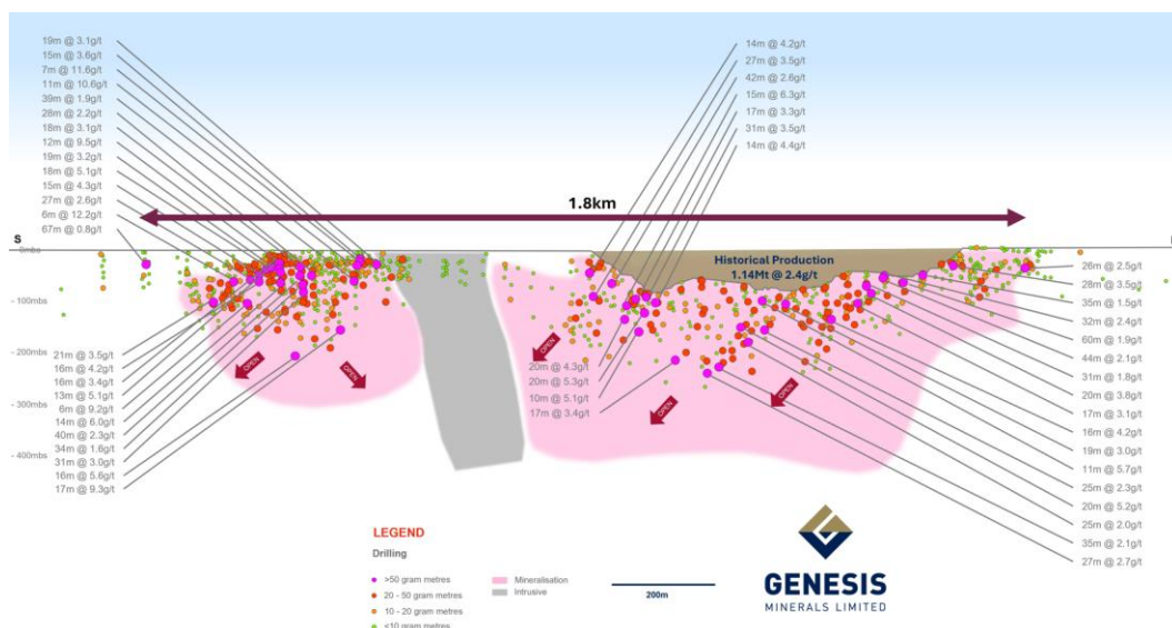
Figure 1. Beasley Creek long section - First cab off the rank*
