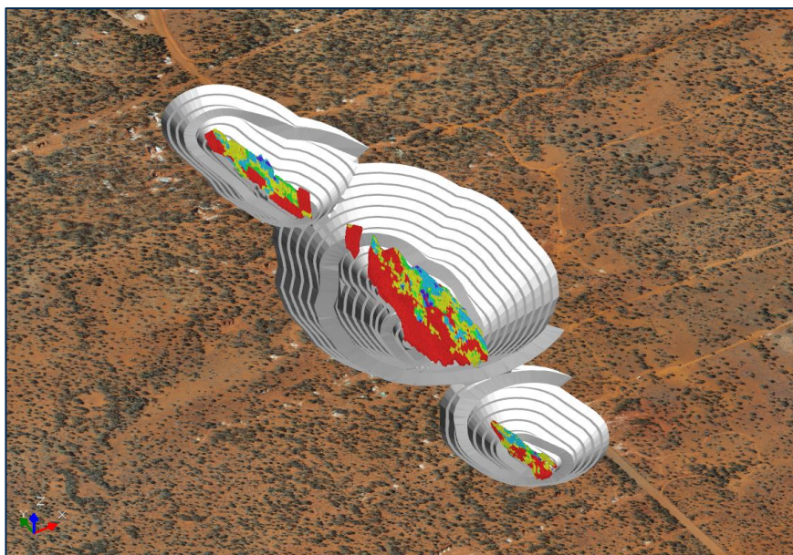
Figure 14. Hub Reserve Pit Designs
