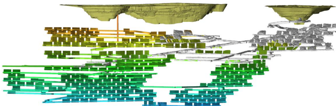
Figure 12. Ulysses Underground Reserve Design
