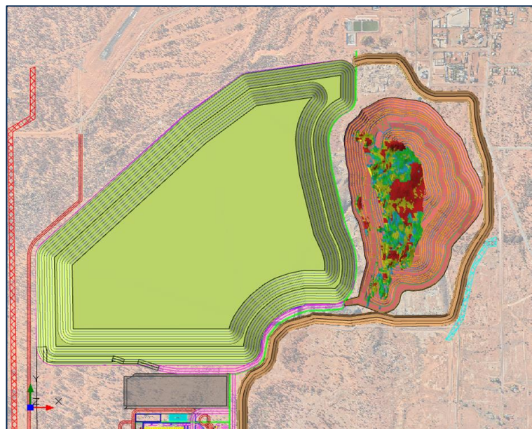
Figure 15. Tower Hill Open Pit LOM
