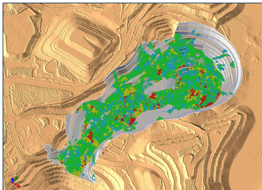
Figure 16. Jupiter Ore Reserve Layout
