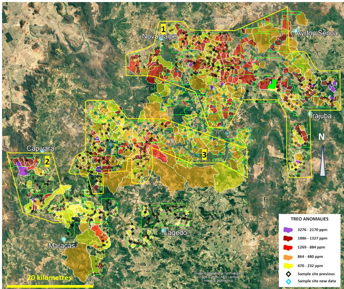
Figure 9. TREO anomalies in the NW Down Under Project from current results and those previously released (ASX 10 October 2024, 9 February 2026).
