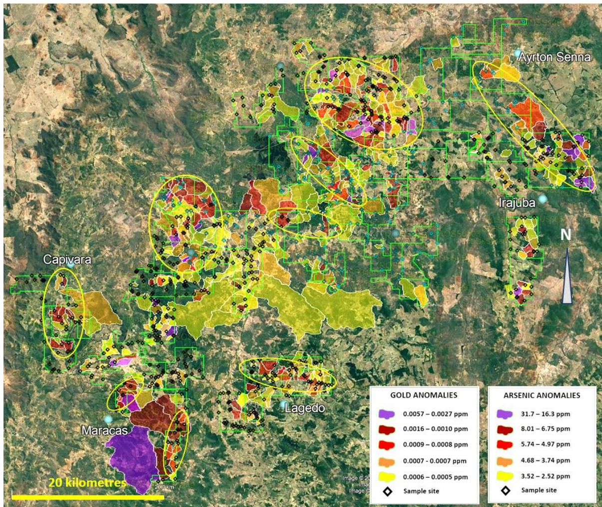
Figure 8. Combined Gold and Arsenic anomalies in the NW Down Under Project from current results and those previously released (ASX 10 October 2024, 9 February 2026).
