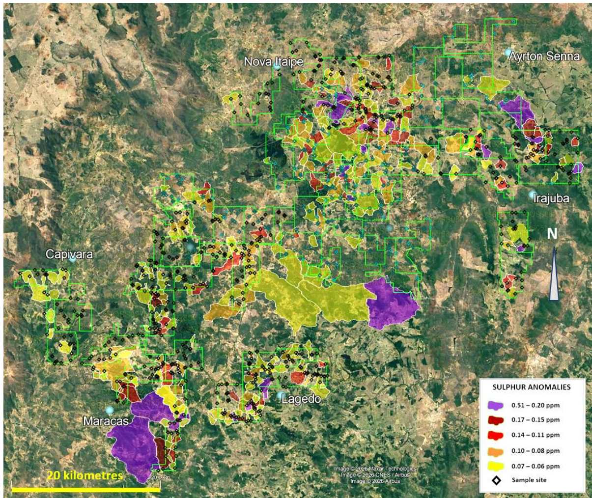
Figure 6. Sulphur anomalies in the NW Down Under Project from current results and those previously released (ASX 10 October 2024, 9 February 2026).
