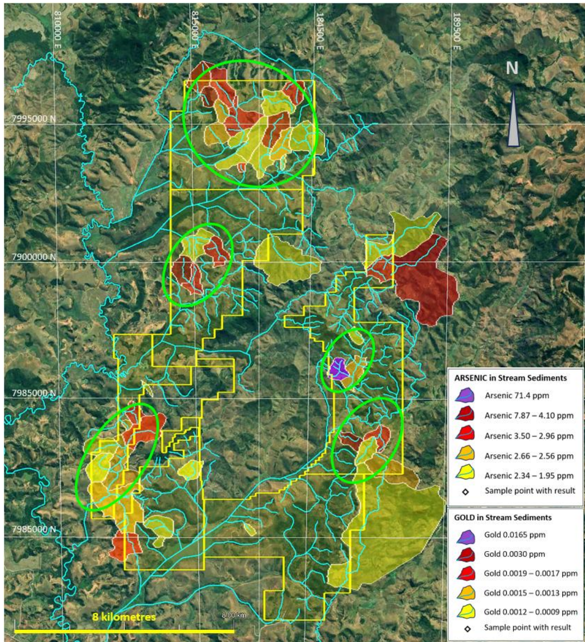
Figure 9. Gold targets of the Franciscopalis prospect area defined by combined gold and arsenic anomalies.
