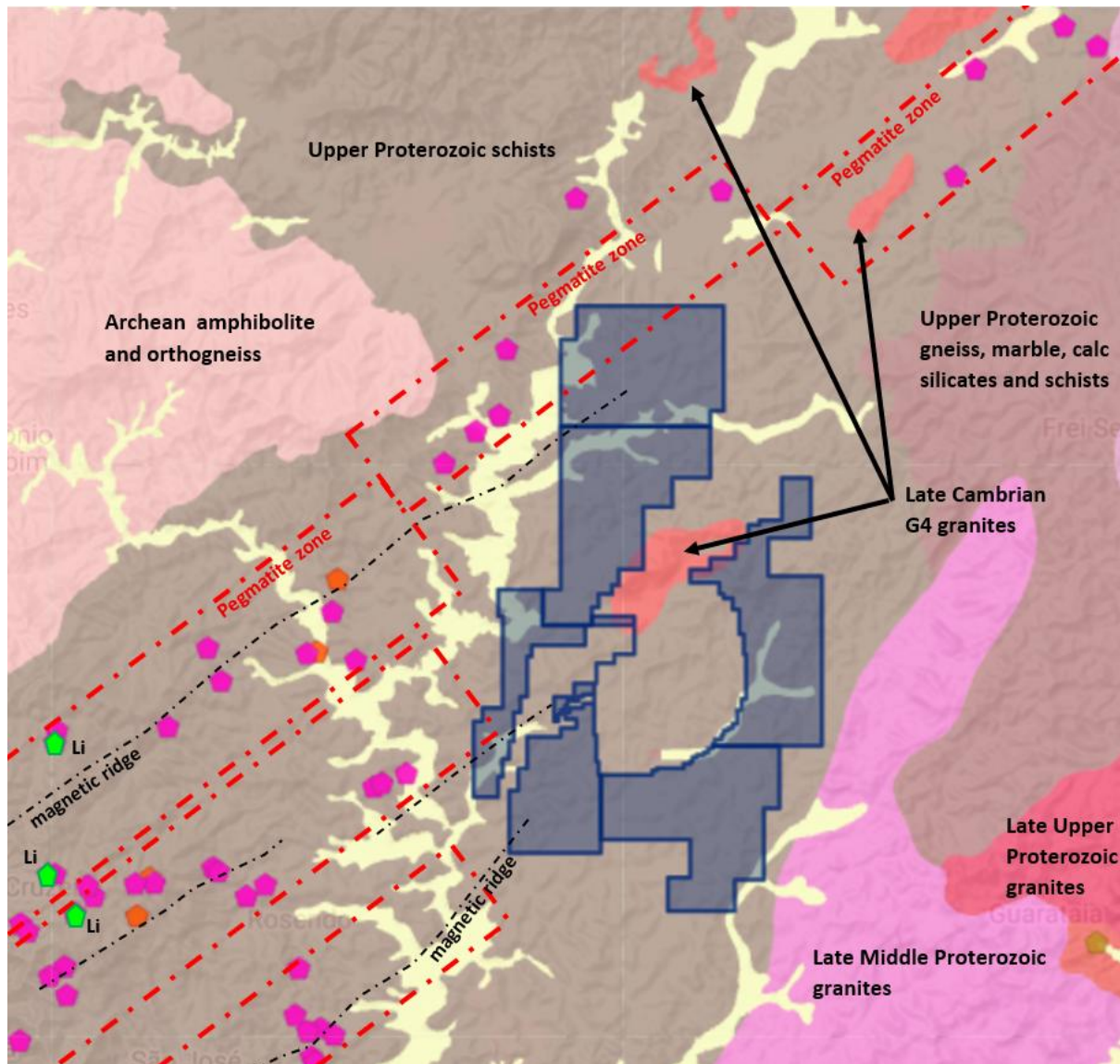
Figure 10. Geology at 1 million scale of the Franciscopalis Project area. Interpreted magnetic ridges are shown together with pegmatite mineral occurrences. Minerals recorded are mainly quartz, tourmaline, beryl, some niobium, and Mn bearing beryl, indicating evolved pegmatite compositions, but also include three lithium bearing pegmatites to the southwest and one to the northeast off the map along the structural trends defined by the magnetic ridges.
