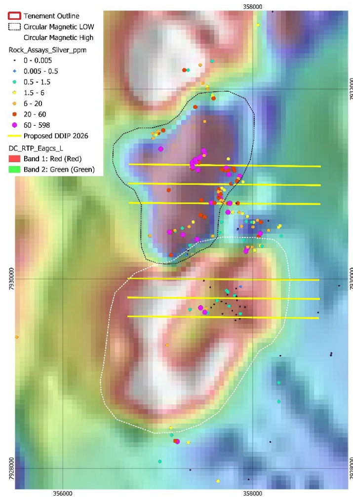
Figure 2: Airborne Magnetic Image showing magnetic anomalies, silver in rock chips and proposed DDIP survey layout (yellow lines).
