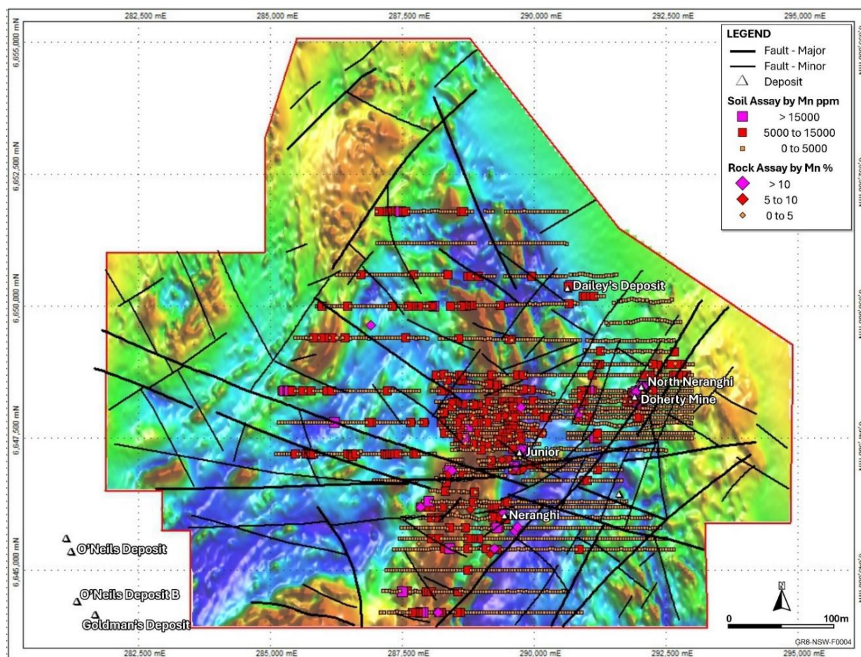
Figure 4: Geochemical sample data (with scaled >5,000 Mn ppm size symbols as indicated) 4 , over RTP (reduced to the pole) magnetics and interpretation. Note strong NE trend associated with the Doherty Mine and North Neranghi deposit. The potential extensions of this mineralisation will form part of the proposed drilling program of the Doherty mine area.
