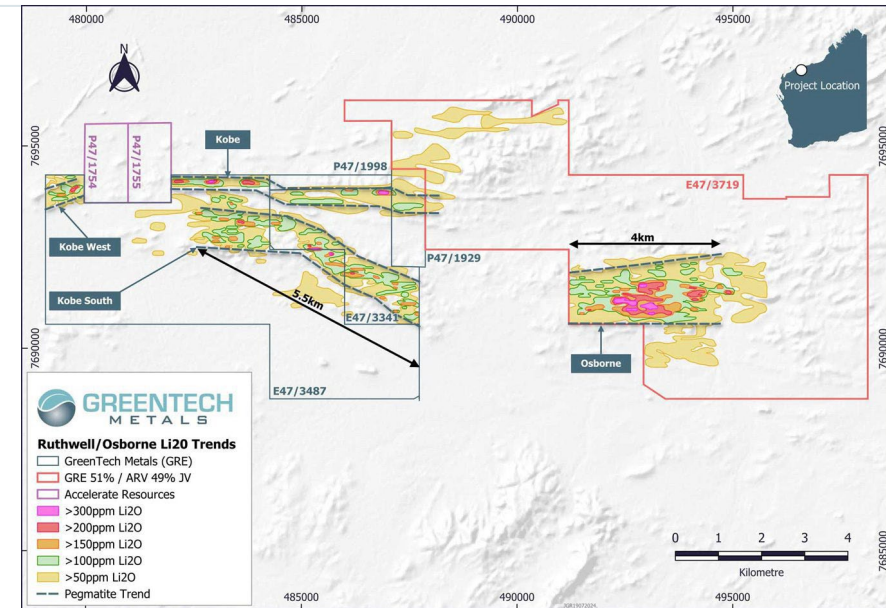
Lithium soil trends at Kobe and Osbourne
