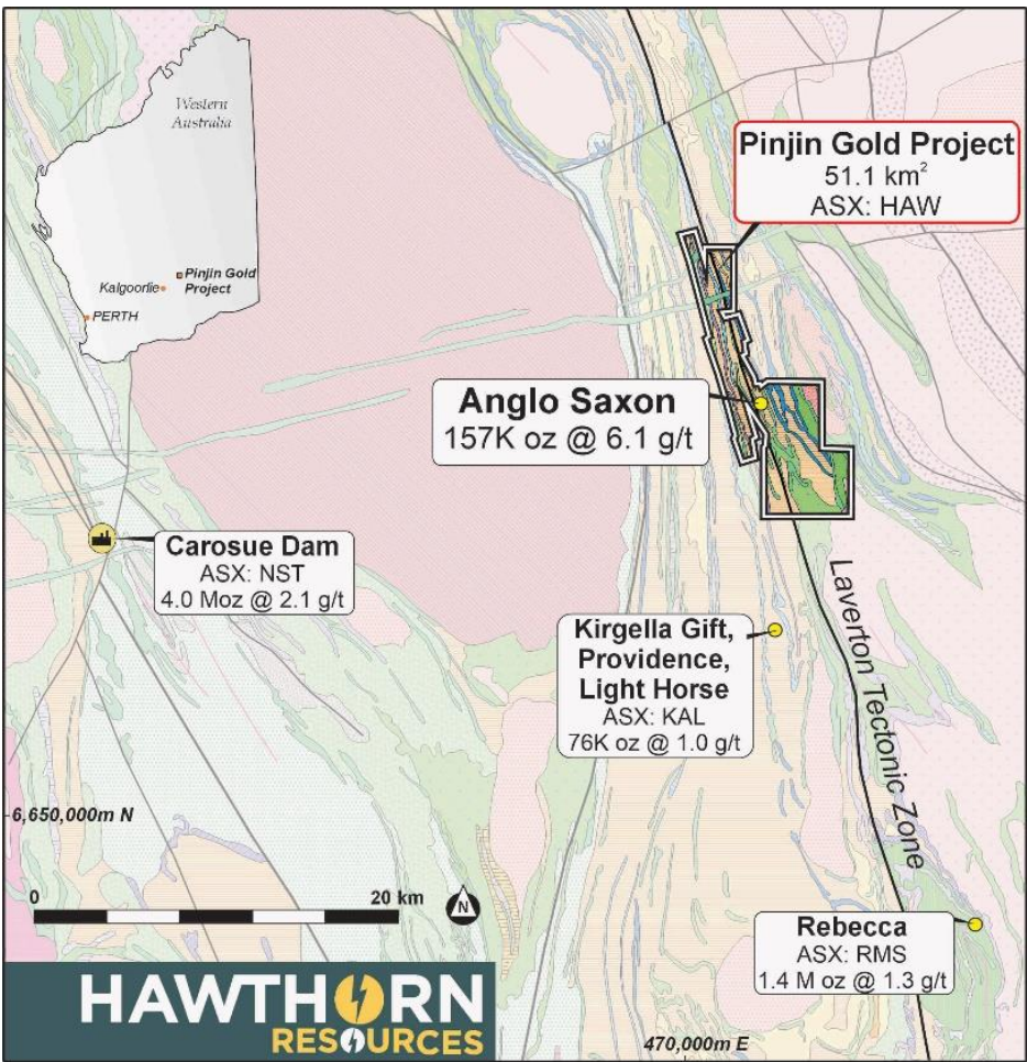
Anglo Saxon Gold Project in Western Australia
