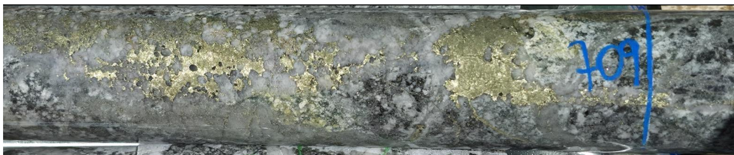
Core photo from DKD039 (709m downhole) showing vein-hosted and disseminated chalcopyrite (~3%) and pyrite (~2%) mineralisation in strongly veined tonalite host rock, assay results expected April 2026¹
