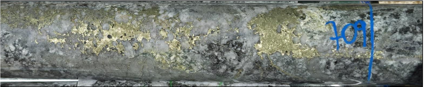
Core photo from DKD039 (709m downhole) showing vein-hosted and disseminated chalcopyrite (~3%) and pyrite (~2%) mineralisation in strongly veined tonalite host rock, assay results expected April 2026 1
