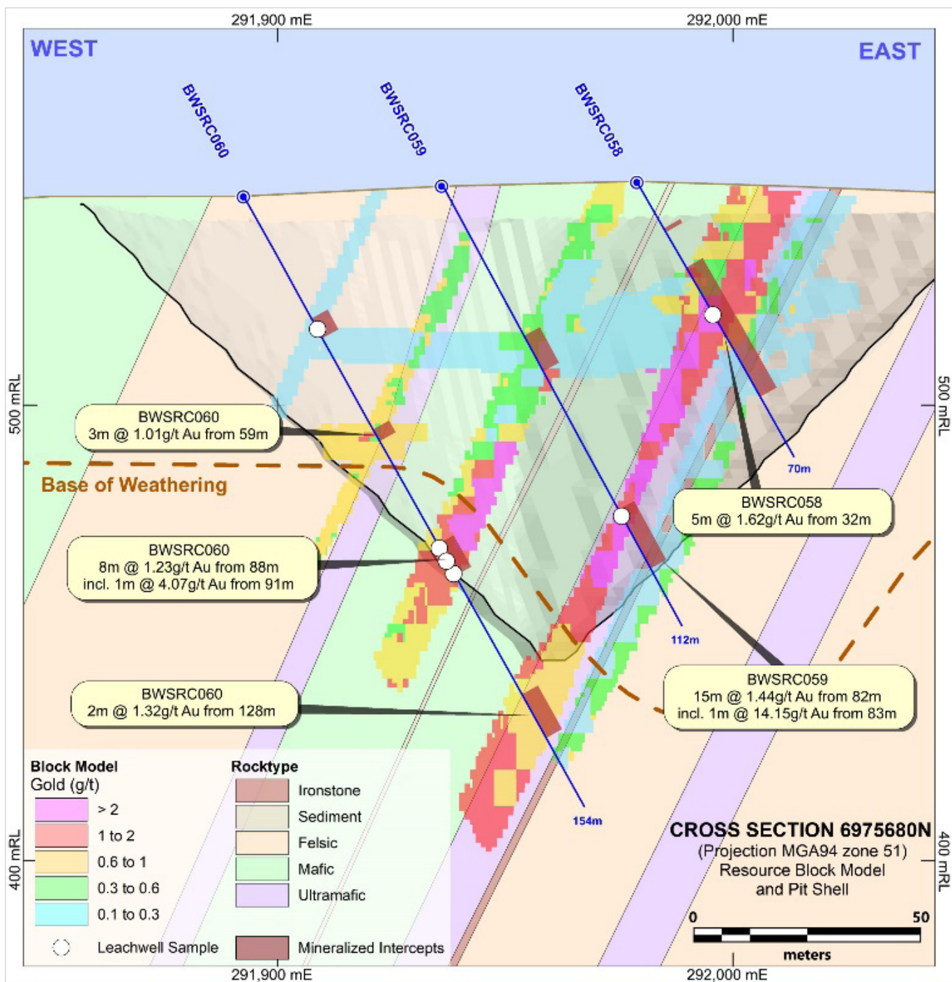
Section 3975680 with leach samples. Oblique view looking north-west showing drilling and block model with optimised pit.
