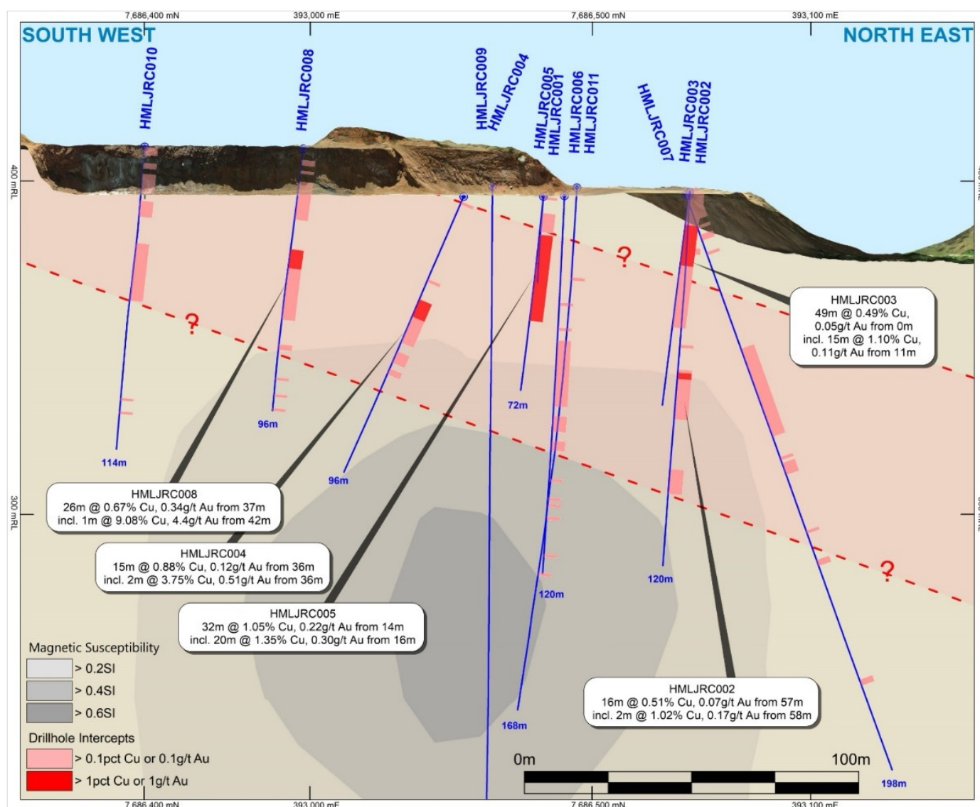
Lady Jenny Long Section showing drill-hole traces, copper and gold assay results with the magnetic anomaly tested by HMLJRC009.
