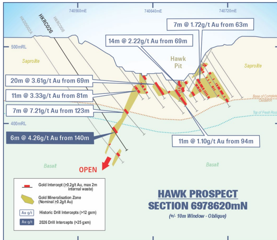
Figure 5: Hawk cross section showing interpreted mineralised zones, 2026 RC intercepts (>25 GxM) and historic intercepts (>12 GxM) labelled.
