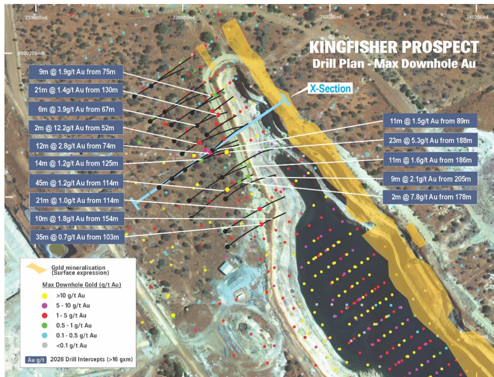
Figure 2: Kingfisher drill hole plan showing all drill collars coloured by maximum downhole gold (g/t Au) and recent drill hole gold intercepts (>16 GxM) over satellite image.
