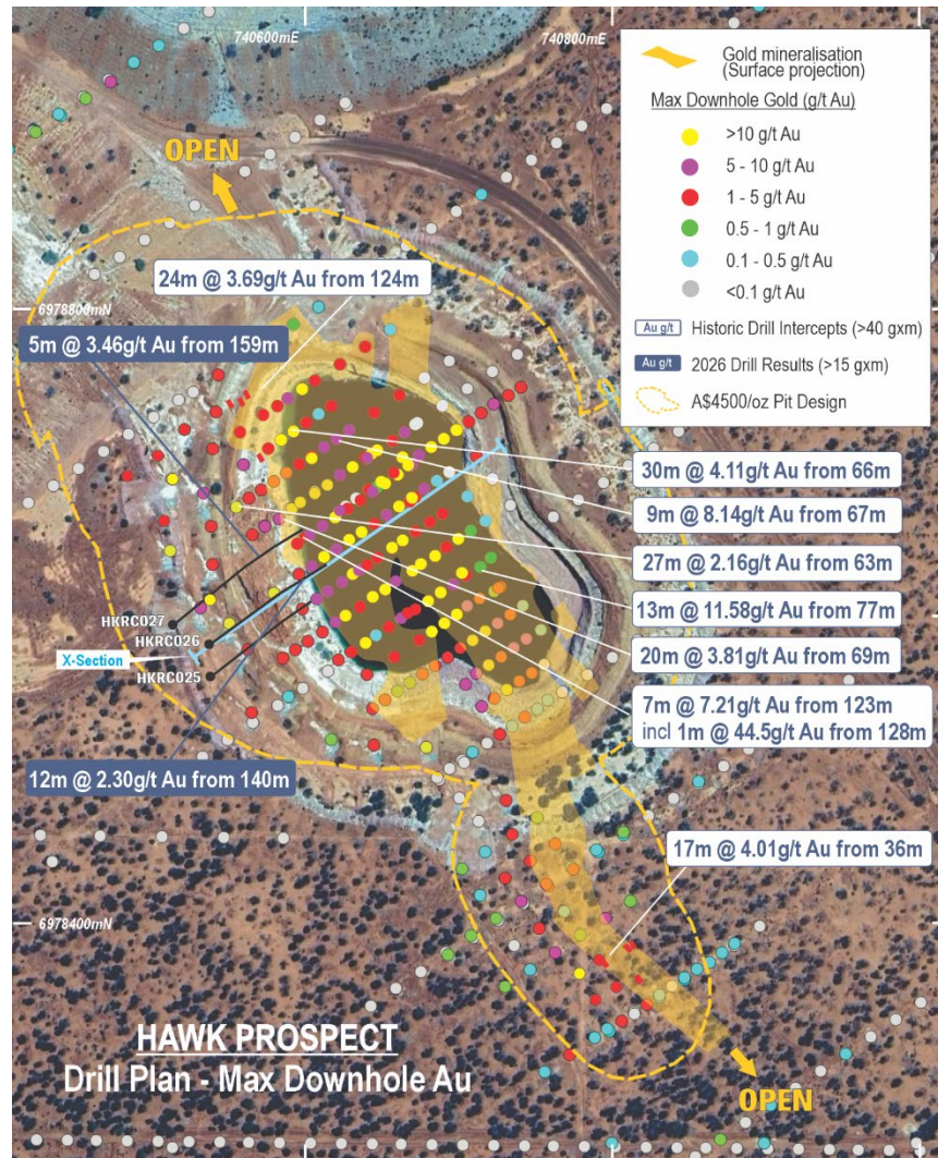
Figure 4: Hawk drill hole plan showing all drill collars coloured by maximum downhole gold (g/t Au), recent gold intercepts (>15 GxM) and historic intercepts (>40 GxM) over satellite image.
