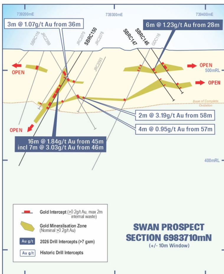
Figure 7: Swan cross section showing interpreted mineralised zones and recent (>7GxM) intercepts and historic intercepts (>3 GxM) labelled.
