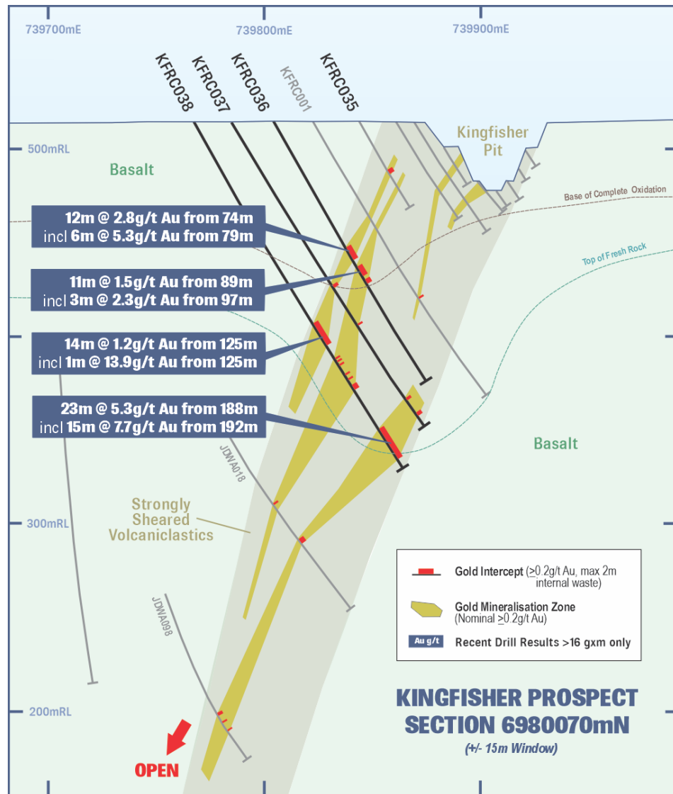
Figure 3: Kingfisher cross section showing recent RC drilling intercepts (>16 Gxm), interpreted geology and mineralised envelope and Kingfisher open pit.
