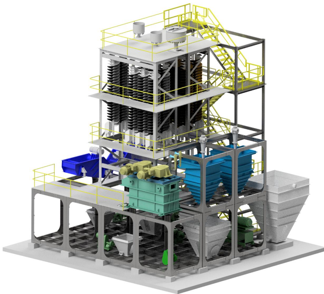
Figure 2 – IHC Modular Wet Plant Design (50kt final product per annum)
