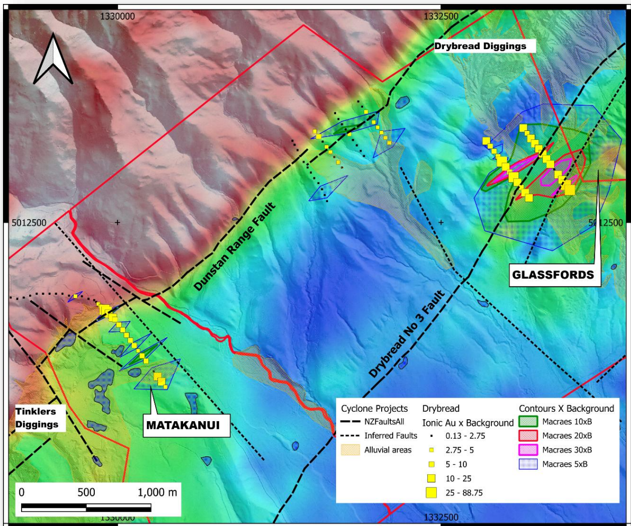
Figure 9. Gold and Pathfinder geochemical responses overlaid on 390Hz resistivity and Lidar topography imagery over Glassfords & Matakanaui area
