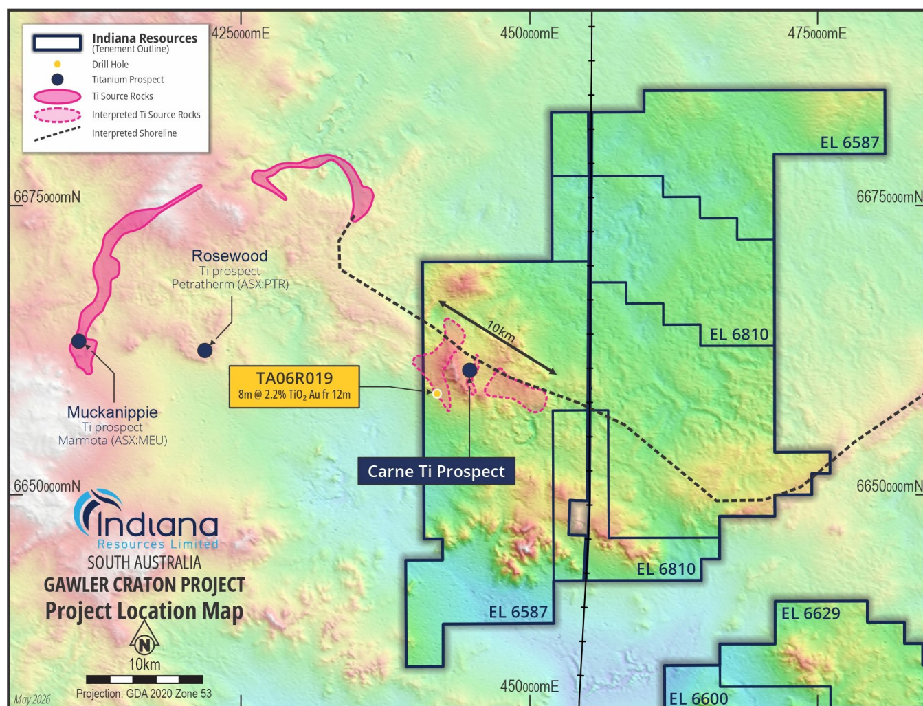
Figure4: Interpreted Paleo Shoreline over digital terrain model and HM prospects
