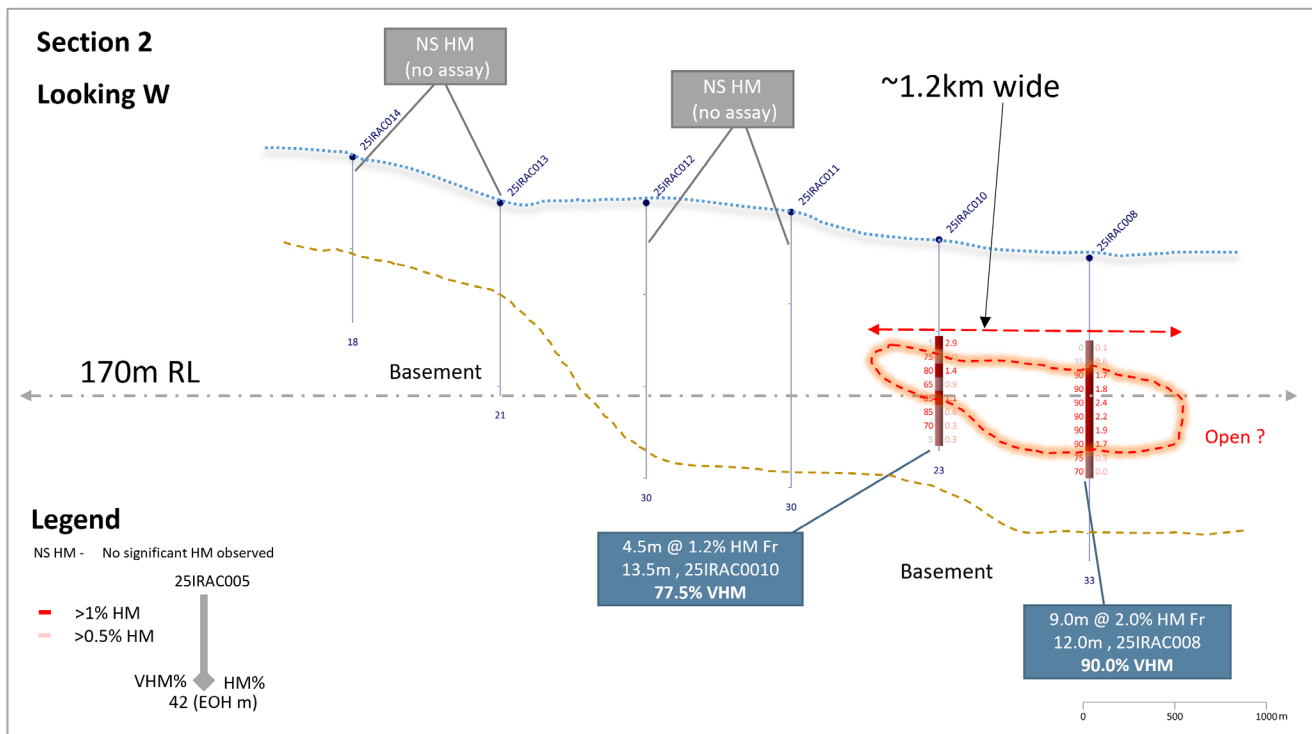
Figure 5: Drill hole cross-section Section 2 for HMS drilling program, Irria Prospect.
