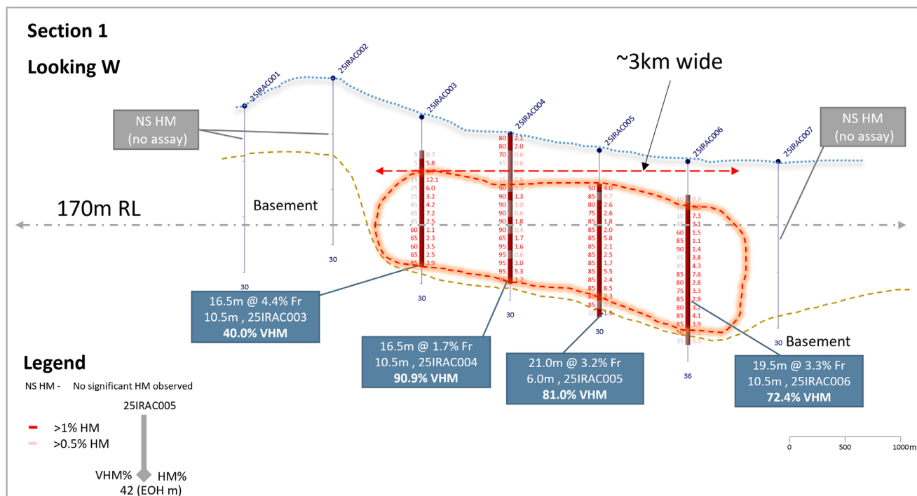
Figure 4: Drill hole cross-section Section 1 for HMS drilling program, Irria Prospect.
