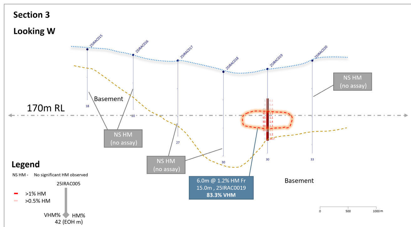
Figure 6: Drill hole cross-section Section 3 for HMS drilling program, Irria Prospect.
