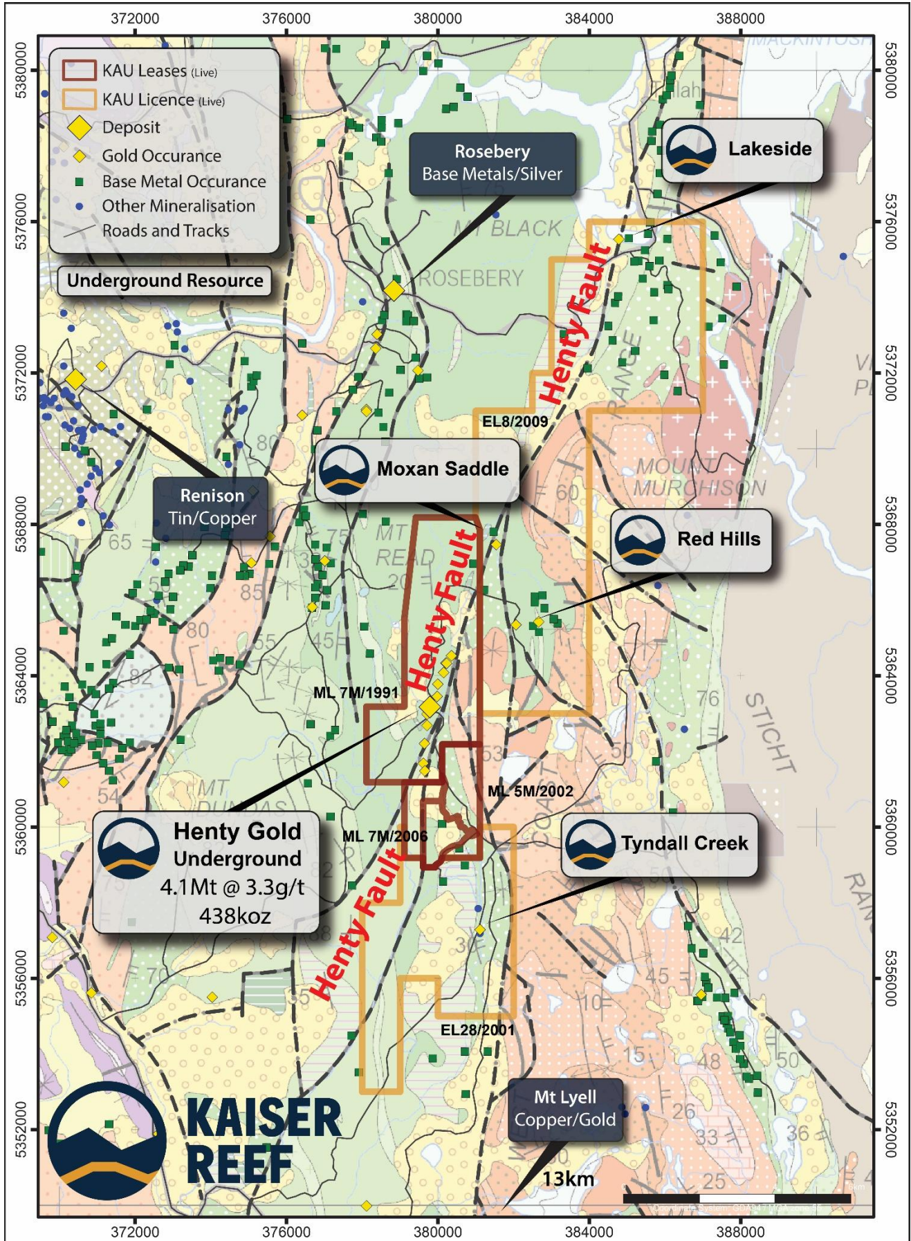
Figure 1. Henty Project with gold and base metal targets and neighbouring projects.
