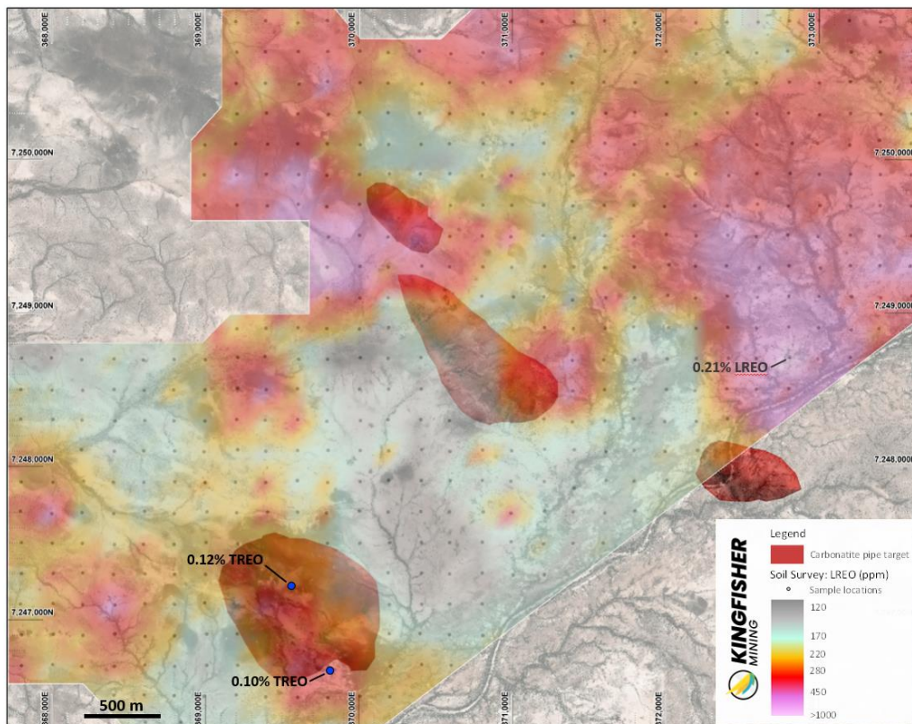
Figure 10: LK1 surface REE geochemistry and carbonatite pipe targets. The REE geochemistry has been calculated from a suite consisting of CeO 2 , La 2 O 3 , Nd 2 O 3 and Pr 6 O 11 . The carbonatite pipe targets were derived from three-dimensional modelling of the combined magnetics and gravity geophysics data. Anomalous rock chip results associated with the southwestern carbonatite pipe target as well as the peak soil geochemistry value of 0.21% LREO are also shown (see ASX:KFM 7 December 2023).
