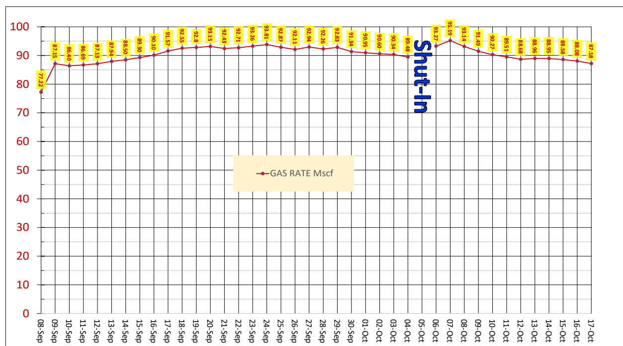
Figure 1: Production Test Well 271-KA03PT10 daily gas flow rate.
