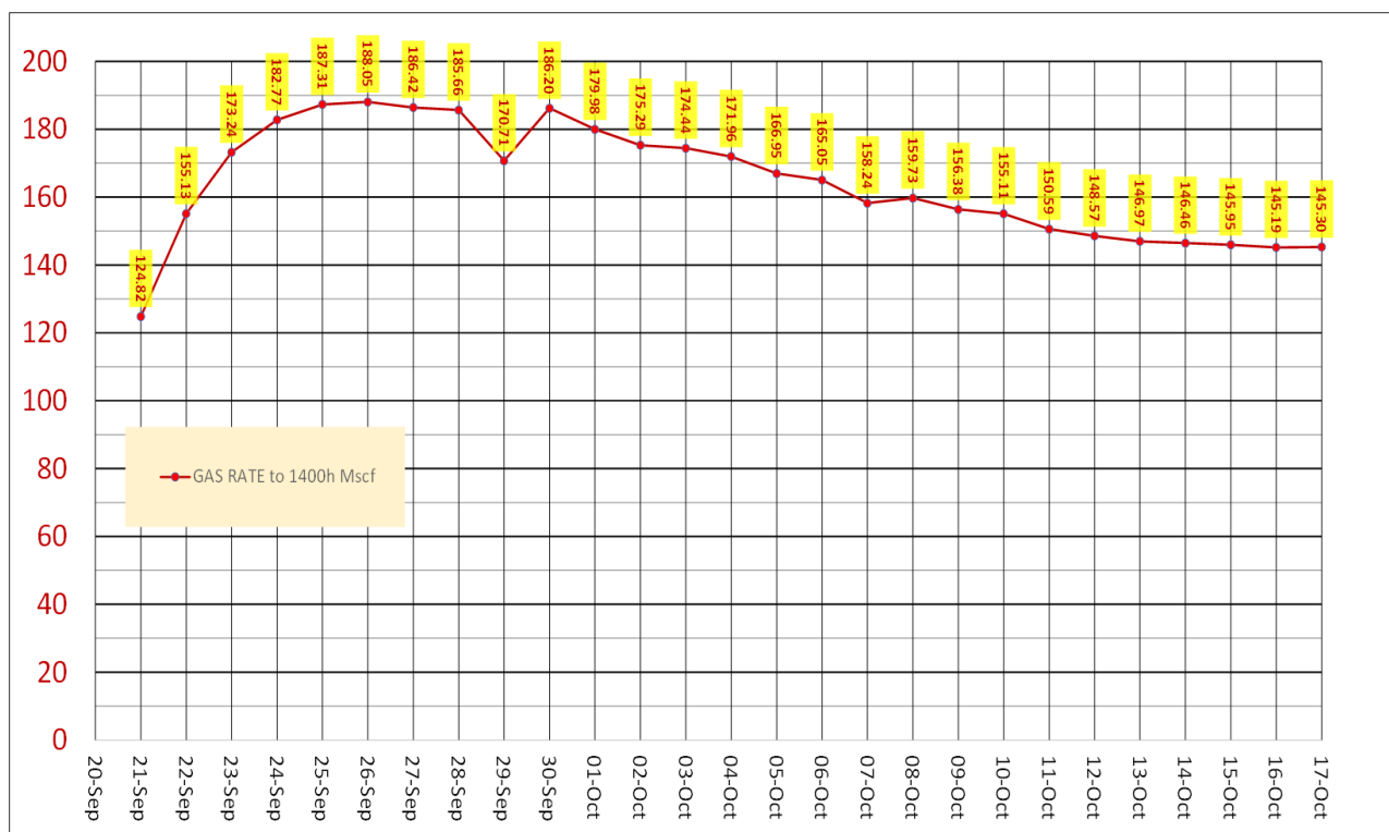
Figure 2: Production Test Well 271-KA03PT06 daily gas flow rate.
