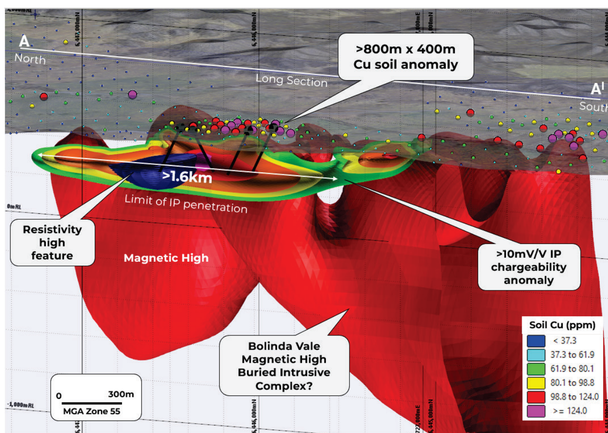
Figure 1. Oblique view looking North-East of long section A to A' displaying planned drillholes (black traces) with coincident Bolinda Vale DDIP chargeability isosurfaces (>10mV/V), resistivity high feature, soil Cu (ppm) with 3D modelled magnetic high response extending to depth with satellite image. All coordinates GDA94 MGAz55.
