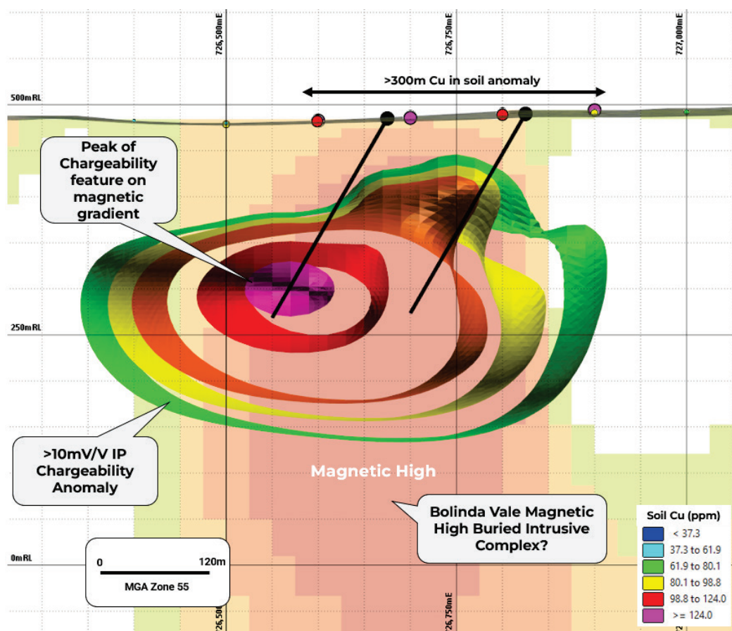
Figure 4. Section B to B' through 6,446,20mN at Bolinda Vale looking North displaying proposed holes (black traces) with DDIP chargeability isosurfaces ( >10\text{mV/V} ), soil Cu (ppm) and 3D magnetic block model. All coordinates GDA94 MGAz55.
