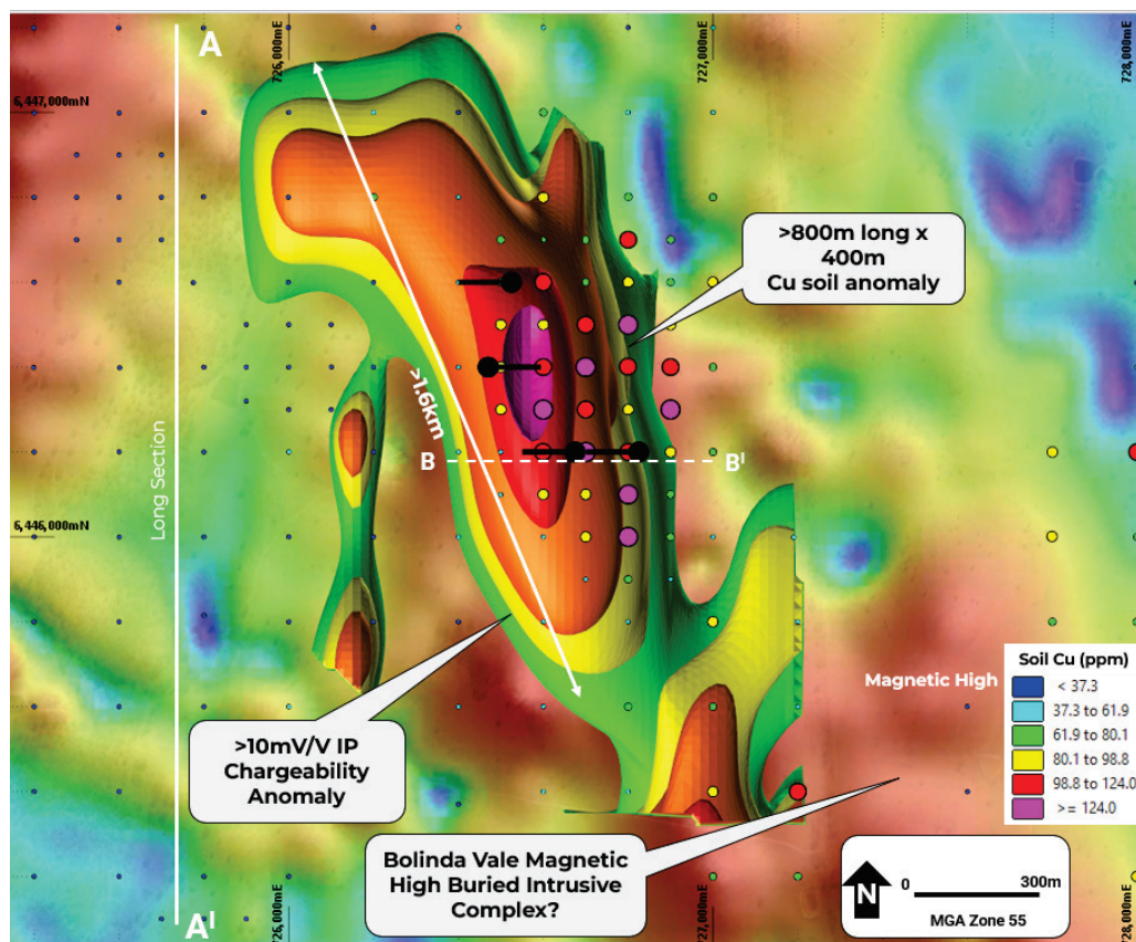
Figure 3. Bolinda Vale DDIP chargeability isosurfaces ( >10\text{mV/V} ), and soil Cu (ppm) on Analytical Signal Magnetic Image with location of long-section A to A' and cross-section B to B'. Note proposed drillholes (black traces). All coordinates GDA94 MGAz55.
