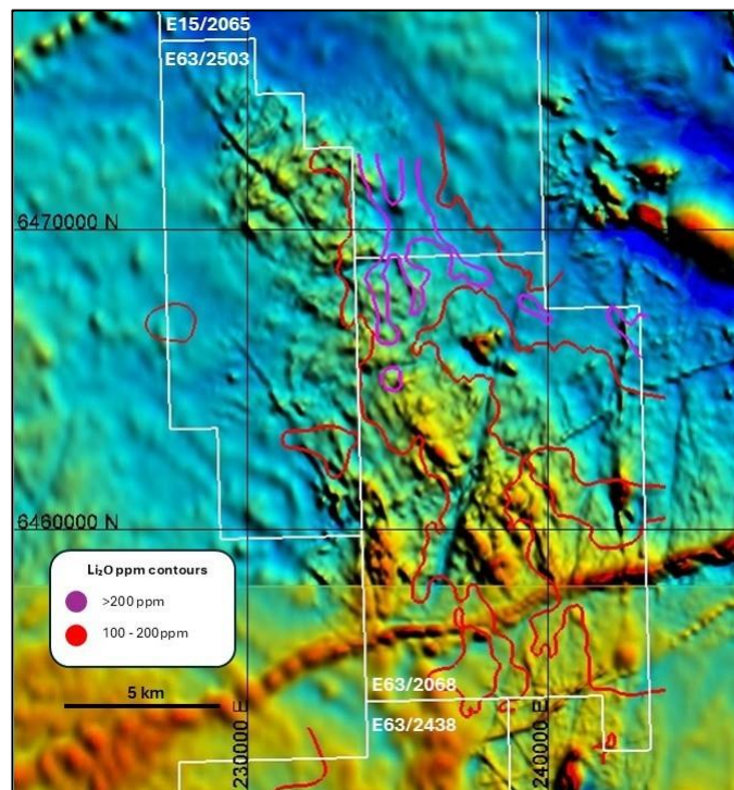
Figure 4: Soil sampling on northern project area showing \text{Li}_2\text{O} contours (overlying total magnetic intensity GSWA 1:250,000)
