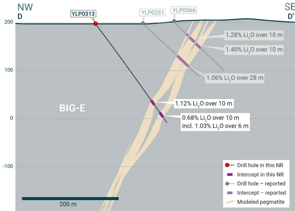
Figure 7 – Section D-D' (refer to Figure 3) looking northeast and showing the BIG East pegmatite. 5
