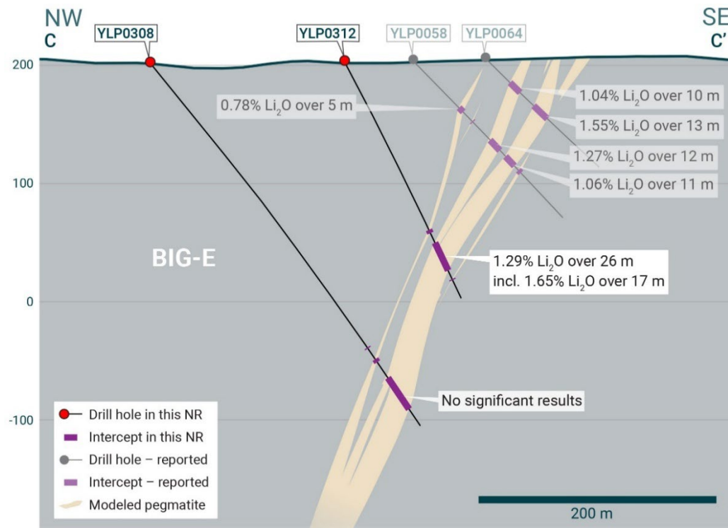
Figure 6 – Section C-C' (refer to Figure 3) looking northeast and showing the BIG East pegmatite. 5
