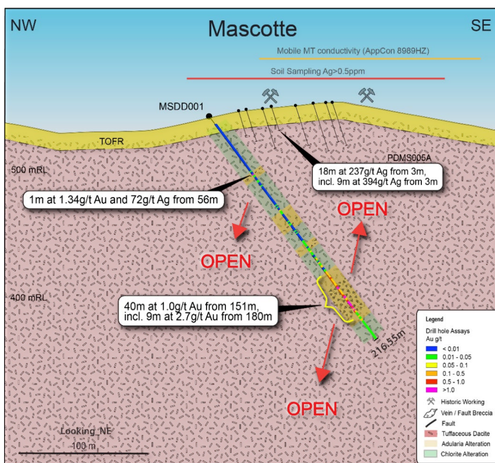
Figure 2. Cross-section of assays of geology interpretation at drill hole MSDD001 ii .
