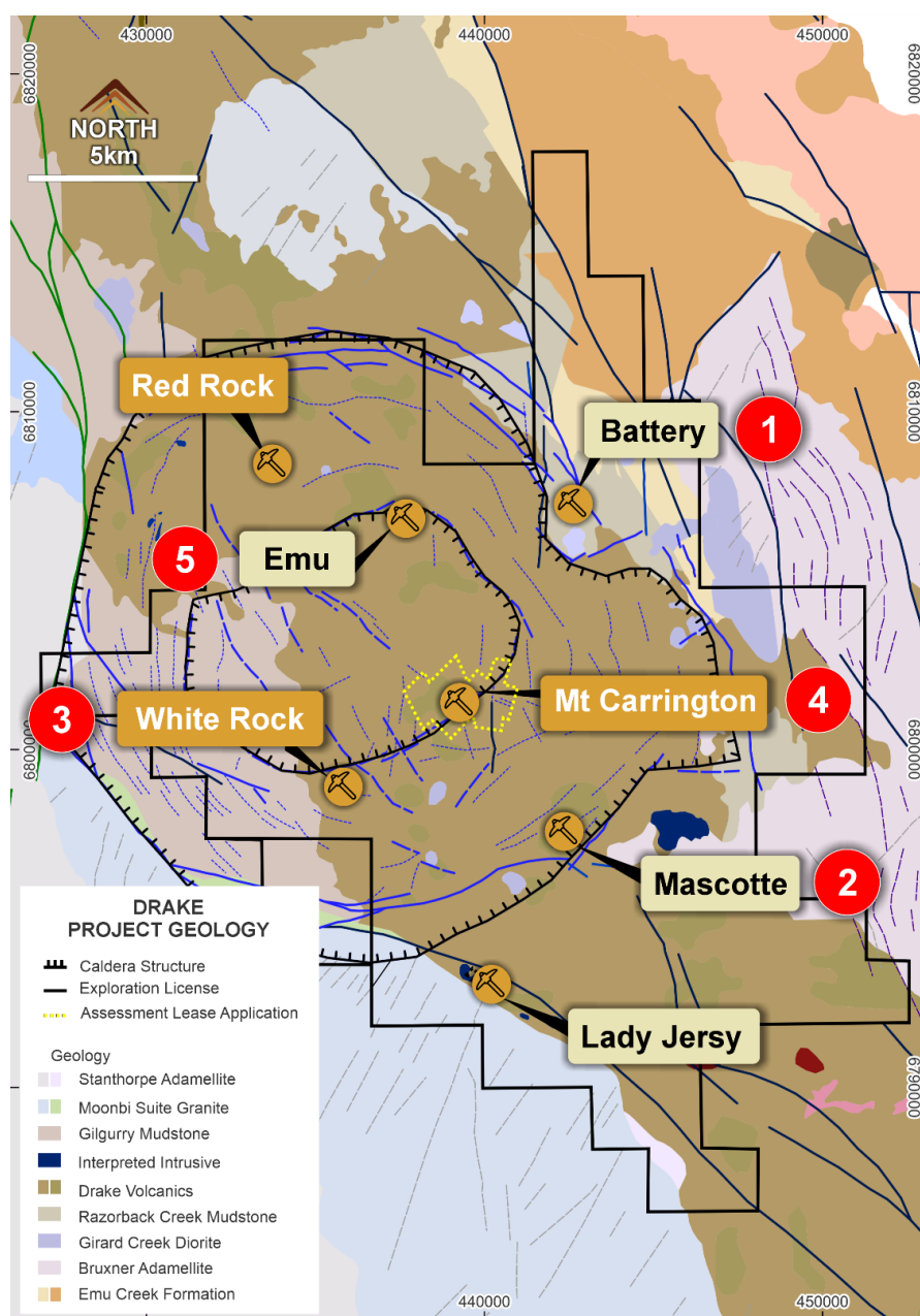
Figure 7. Drake Project Geology and Planned Drilling for 2026 targeting greenfields and brownfields silver, gold, and copper targets.
