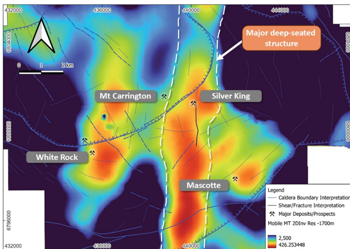
Figure 4. Interpreted deep-set conductive feeder structures and lineaments iii .
