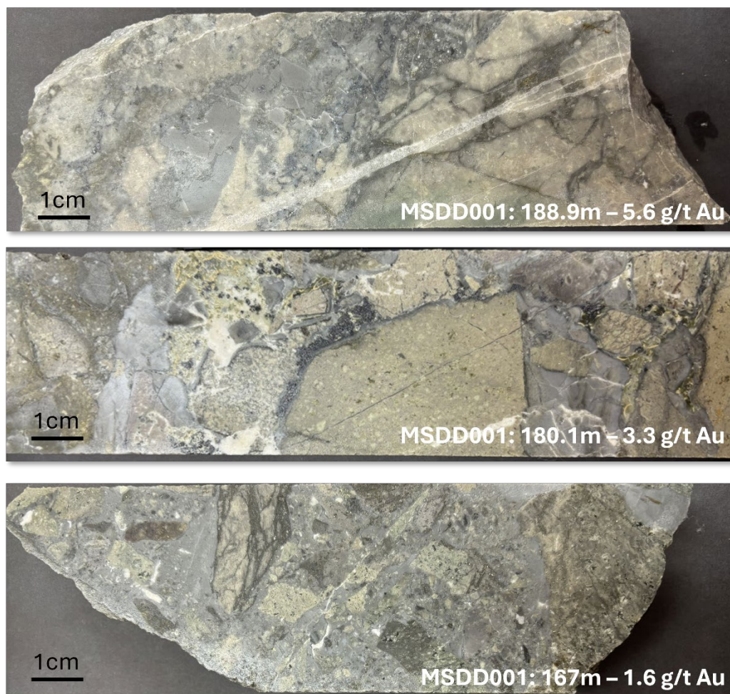
Figure 5. MSDD001 drill core showing patchy, veinlet and disseminated pyrite-sphalerite within chalcedony quartz-carbonate breccia infill.
