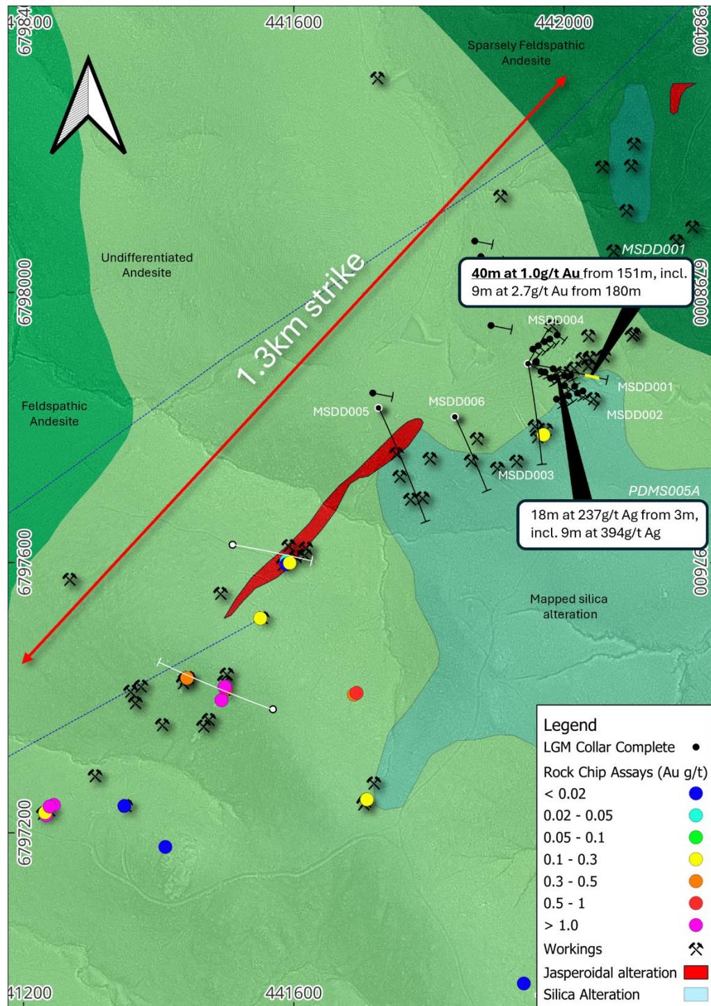
Figure 6. Mascotte Prospect plan view showing rock chip sample gold assay results, completed holes (black dots) planned drilling (white dots), and historical mine workings ii .
