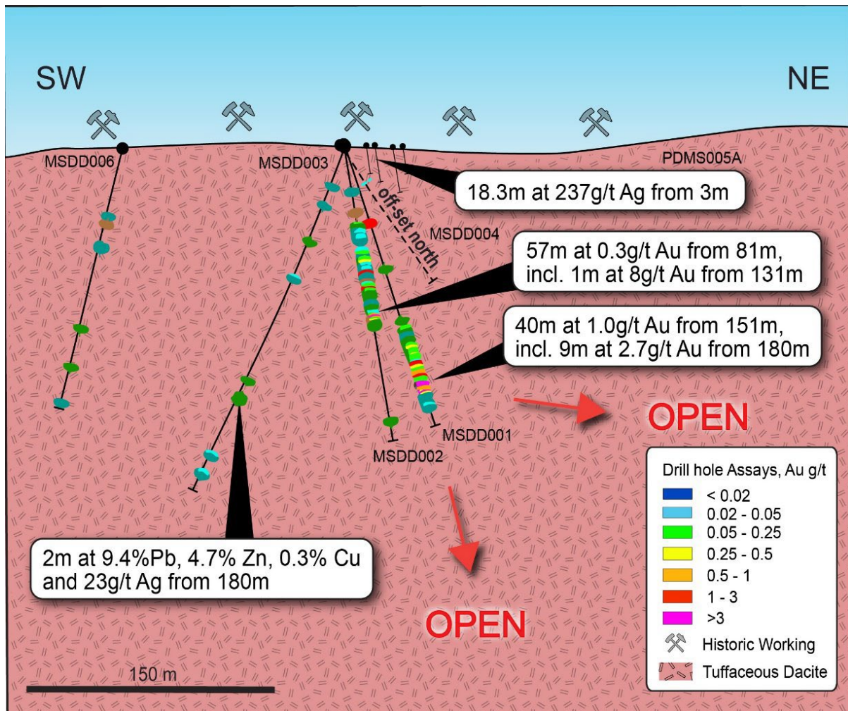
Figure 4: Long-section of the breccia zone at the Mascotte Prospect line of workings.
