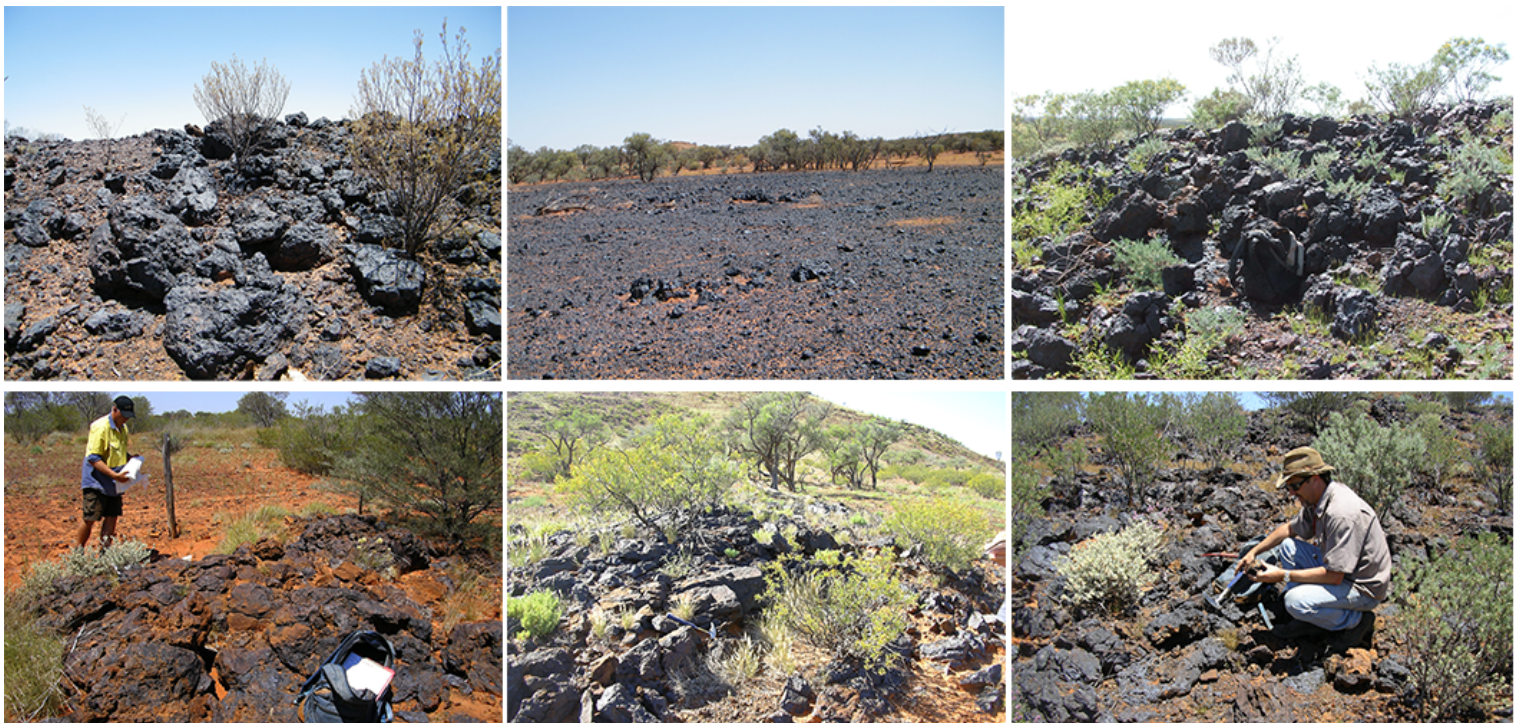
Figure 2 - Some Historical Auvex Sample locations from Lucy Creek areas
