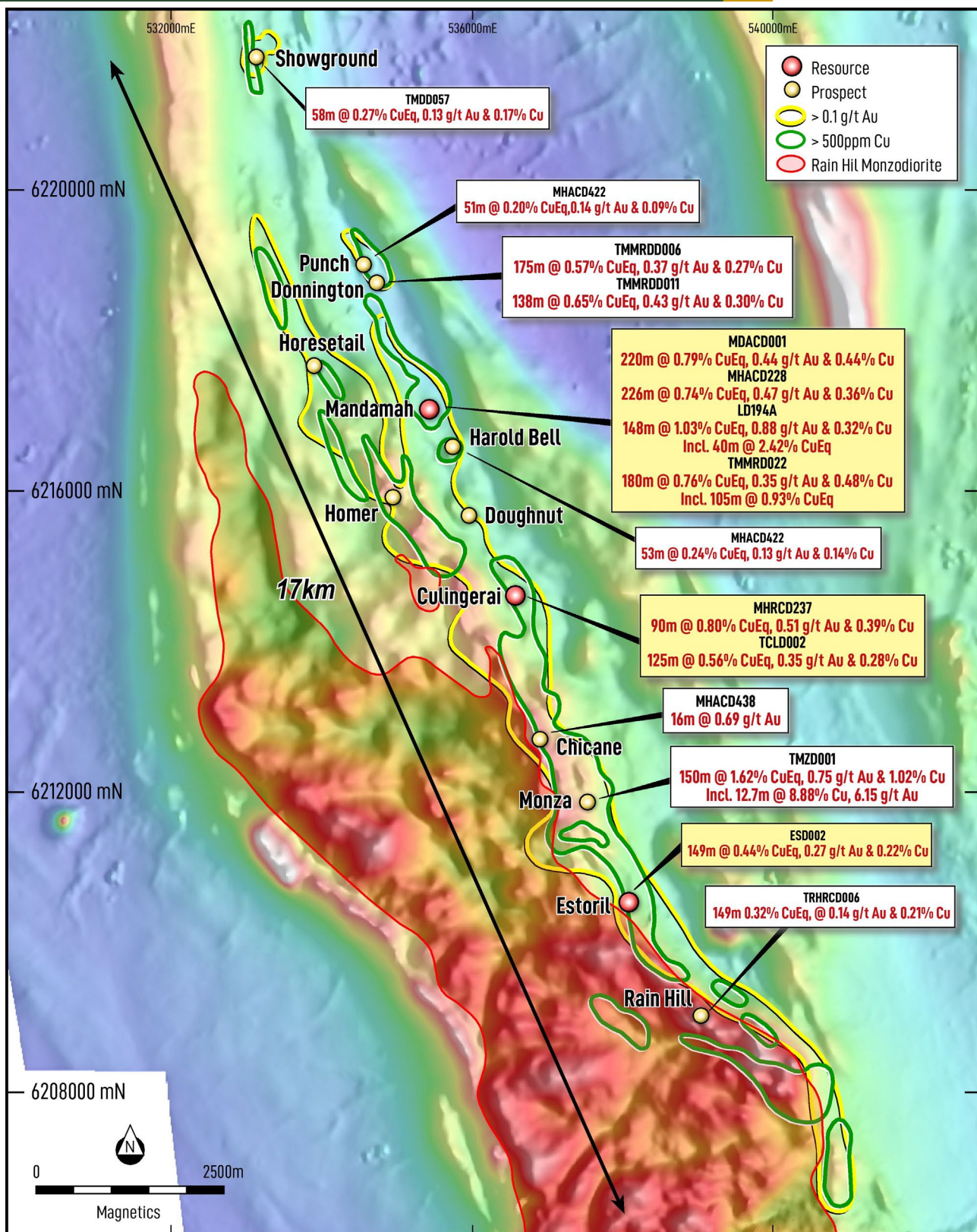
Figure 4: Central Zone resources and prospects over background reduced to pole aeromagnetic image highlighting a 17km strike.
