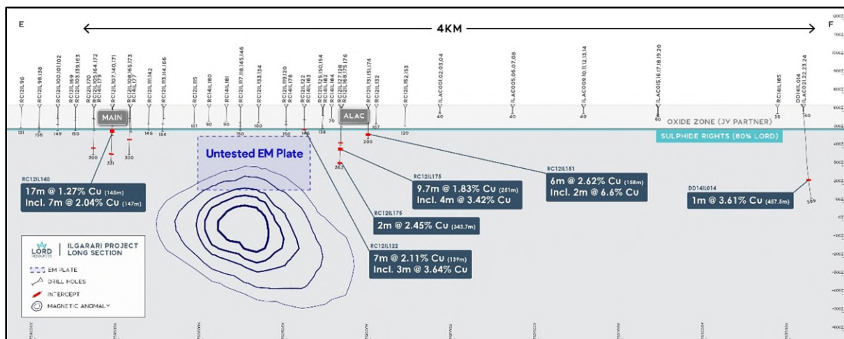
Figure 2 Long Section of EM plate modelling above the magnetic anomaly. Blue lines represent TMI
