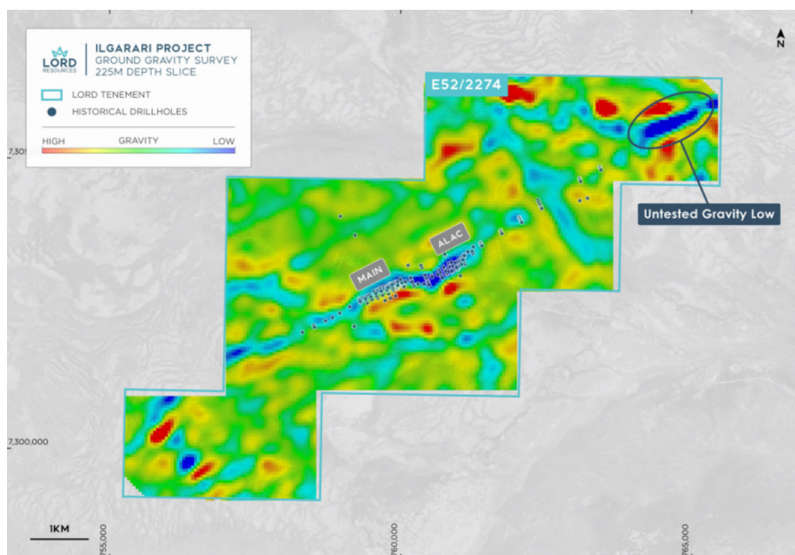
Figure 3 Ilgarari Project, Drillhole collars (black dots) over gravity imagery at 225m depth slice from surface. Blue colours are gravity low, red colours are gravity high
