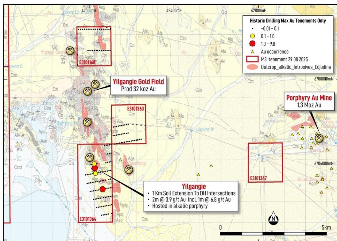
Figure 2. GSWA 1:100,000 Edjudina (3338) Bedrock Geology map Yilgange and Porphyry West prospects
