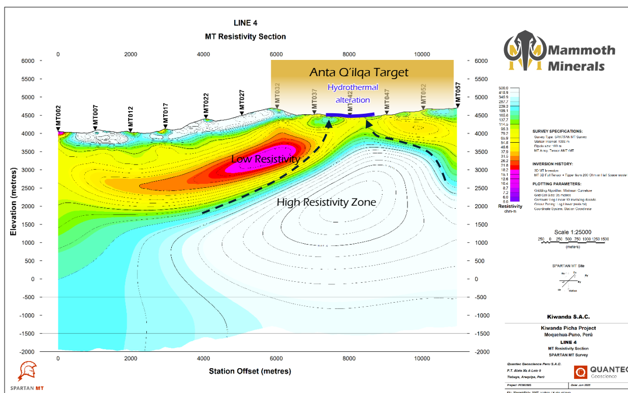
Figure 9: Section highlighting high resistivity vertical structure below the Anta Q'ilqa target.
