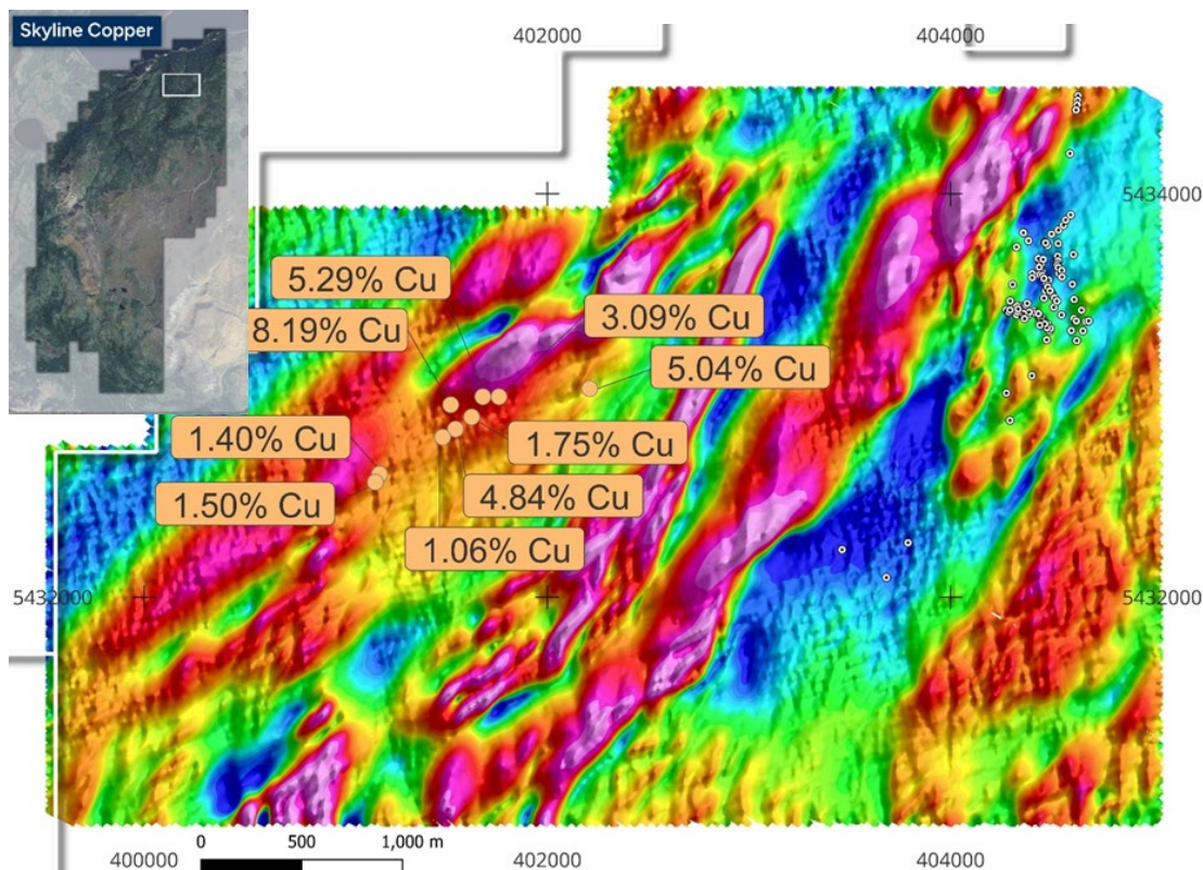
Figure 8: High-resolution magnetics over northern Skyline Tenure with prospecting copper results.
