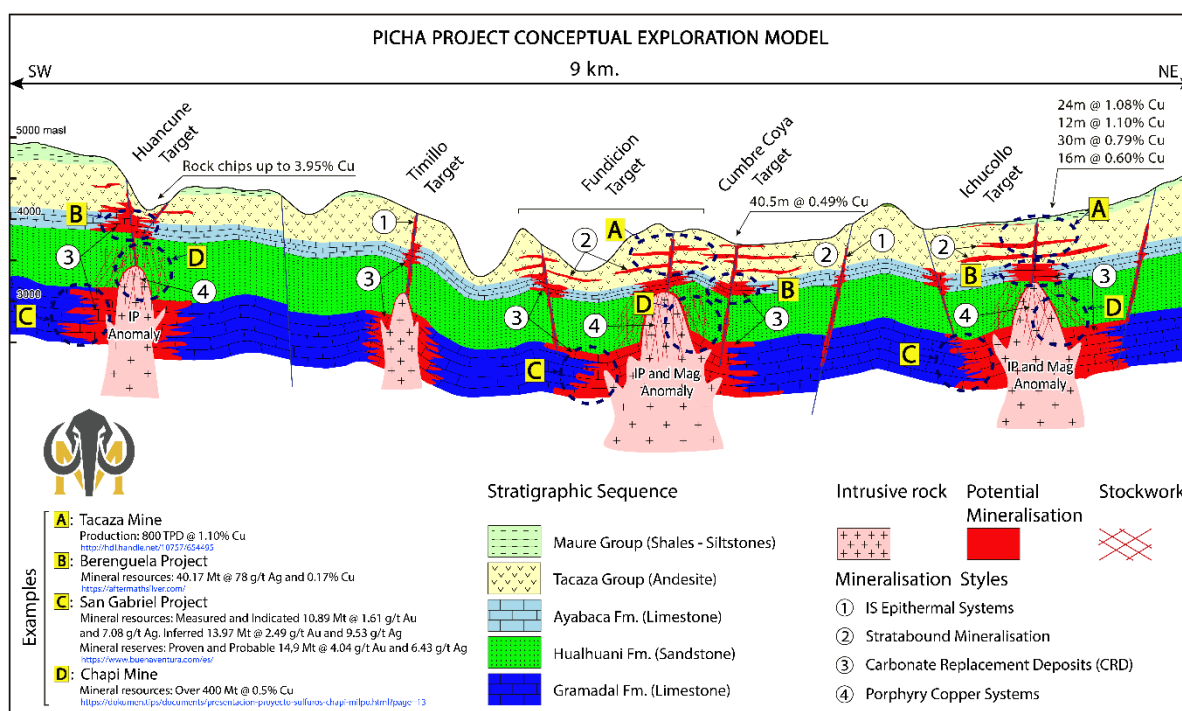
Figure 10: Conceptual cross-section of the Picha Project showing potential mineralisation styles and host stratigraphy.
