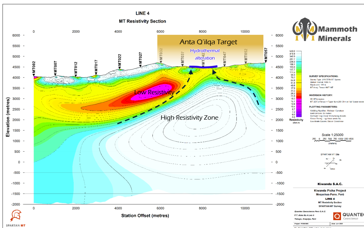
Figure 11: Section highlighting high resistivity vertical structure below the Anta Q'ilqa target.
