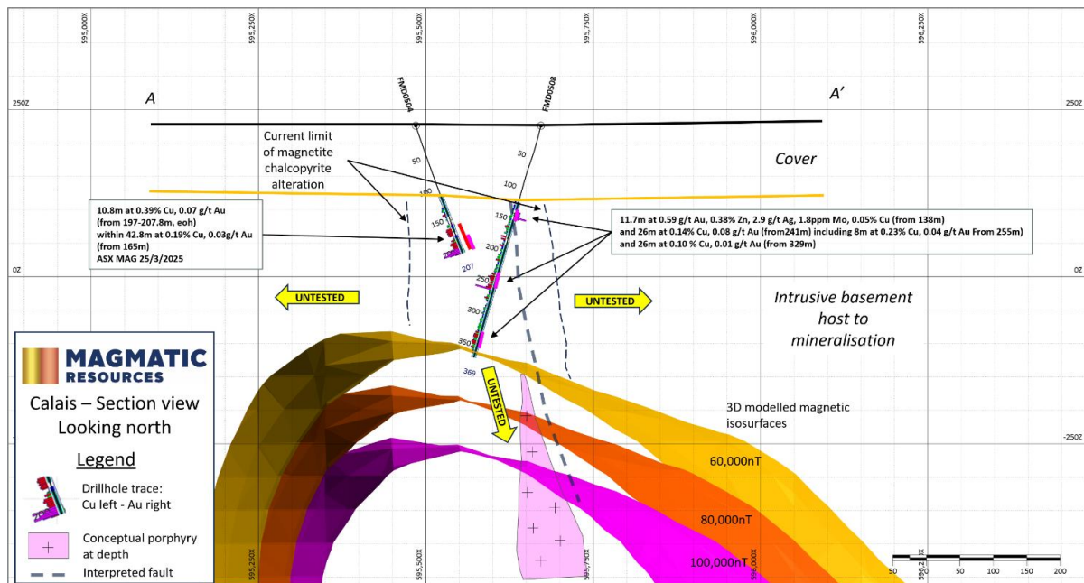
Figure 10. Calais conceptual geological cross section looking north with drilling over 3D modelled magnetic iso surfaces of equal field strength with interpreted magnetite-pyrite-chalcopyrite shell 5
