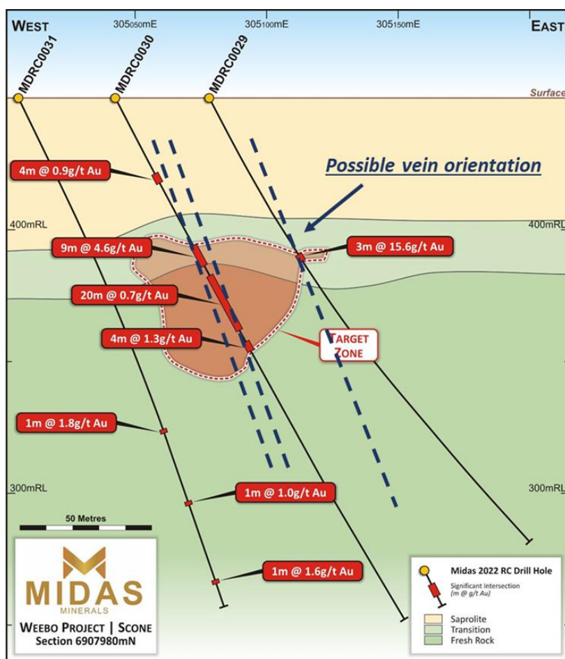
Figure 7: Scone Stone cross-section showing MDRC0029
